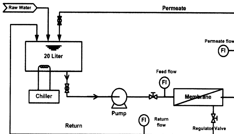
Fig. 1. Schematic diagram of bench-scale cross-flow RO/NF membrane filtration system.
