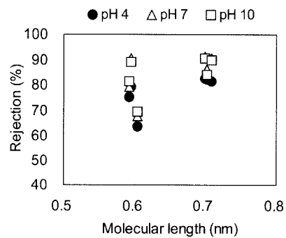
Fig. 5. Removal efficiency as a function of length of solutes for membranes at various pH.
