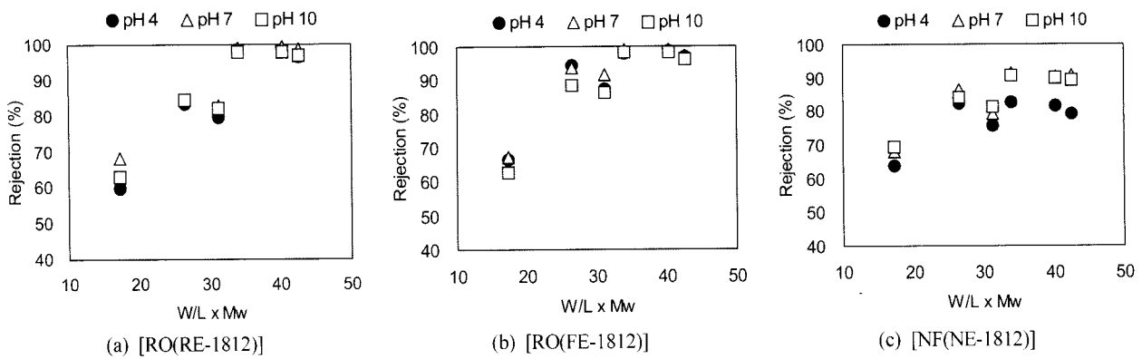
Fig. 7. Removal efficiency as a function of W/L×M w of solutes for membranes at various pH.
