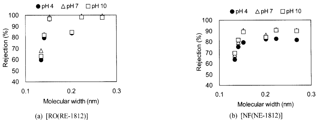
Fig. 4. Removal efficiency as a function of width of solutes for membranes at various pH.
