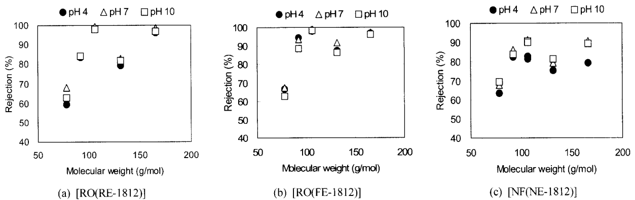
Fig. 3. Removal efficiency as a function of molecular weight of solutes for membranes at various pH.
