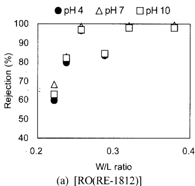
Fig. 6. Removal efficiency as a function of W/L ratio of solutes for membranes at various pH.
