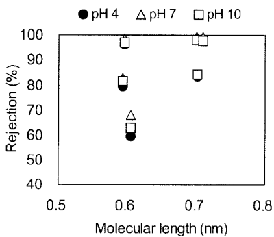
Fig. 5. Removal efficiency as a function of length of solutes for membranes at various pH.
