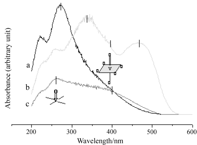
Fig. 5. Diffuse reflectance UV-VIS spectra of (a) VO 2+ -SAPO-5, (b) reference, V 2 O 5 , and (c) VO 2+ -AlMCM-48.
