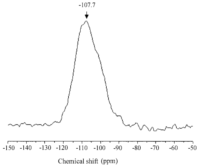
Fig. 4. 29 Si MAS NMR spectrum of calcined VO 2+ -MCM-48 followed by hydration.
