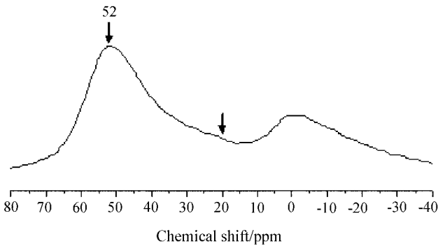
Fig. 2. MAS 27 Al NMR spectrum for calcined AIMCM-48 sample with Si/Al(16) followed by hydration.
