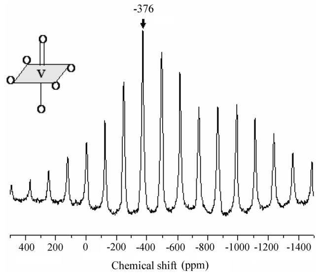
Fig. 3. 51 V MAS NMR spectrum calcined VO 2+ -AIMCM-48 followed by hydration.
