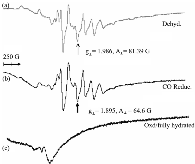
Fig. 6. EPR spectra at 77 K of (a) VO 2+ -AIMCM-48 after O 2 oxidation at 673 K for 5 h follow by dehydration at 873 K for 18 h, (b) after CO treatment at 673 K for 8 h of previously oxidized sample, and (c) after fully hydrated.
