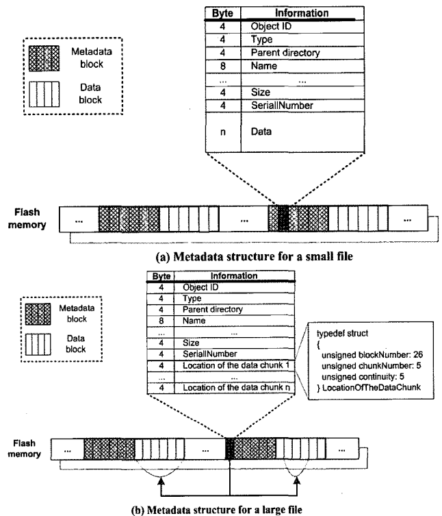
Fig. 5. Management of files using Meta_Data structures
