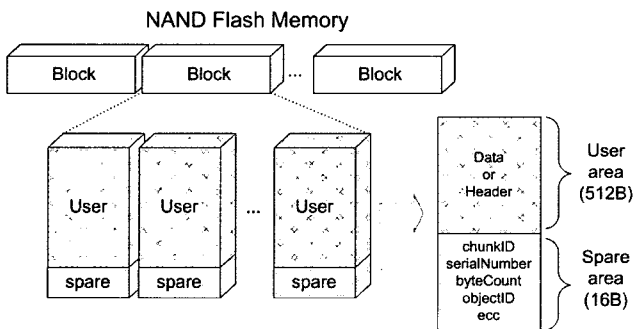
Fig. 2. Flash memory structure of YAFFS
