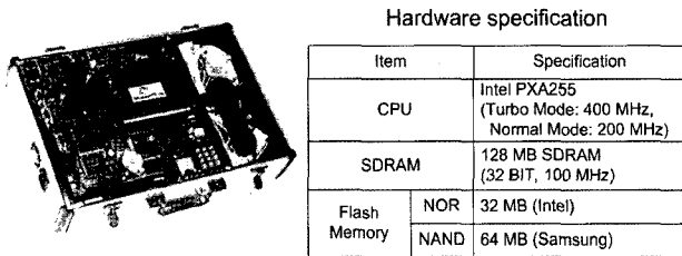
Fig. 8. PXA255-Pro III board specifications
