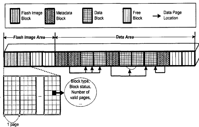
Fig. 4. The proposed flash file system architecture in flash memory
