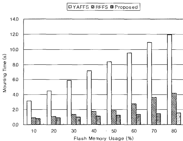
Fig. 9. Mounting time comparison according to flash memory usage
