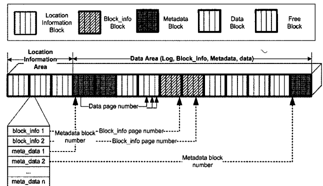
Fig. 3. Flash memory structure of RFFS
