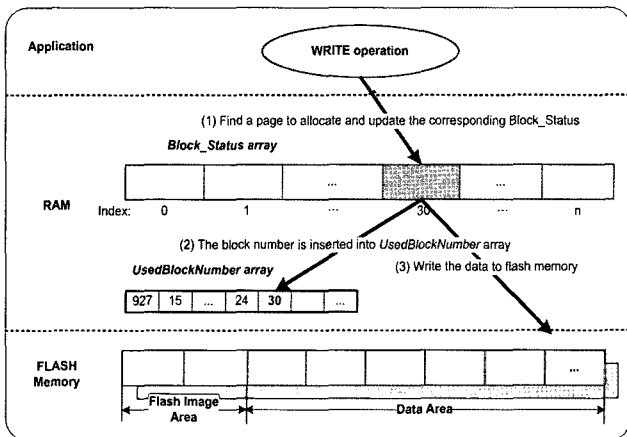
Fig. 6. An example of Block_Status and UsedBlockNumber updates in RAM
