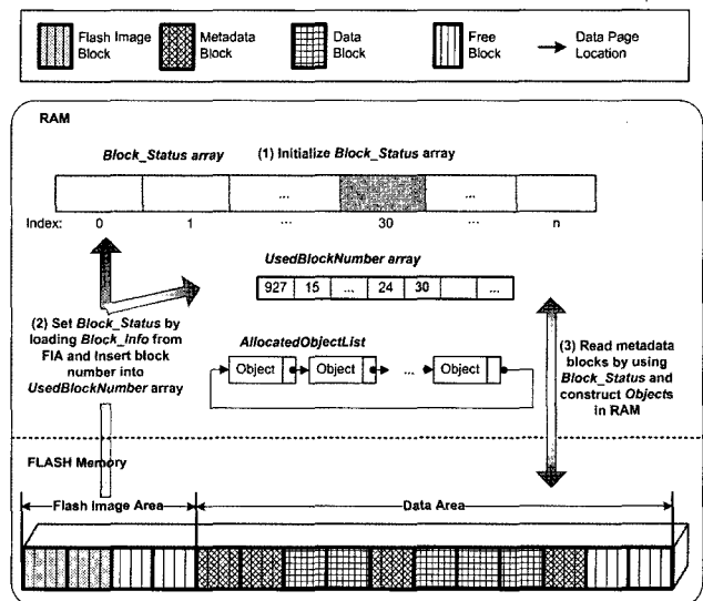
Fig. 7. Mounting procedure of the proposed file system
