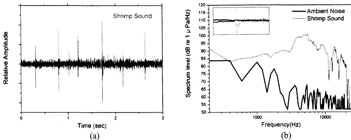
Fig. 7. (a) Typical temporal waveforms of snapping shrimp sound, (b) One click sound and its spectrum. The snapping shrimp sound (solid line) is compared to the usual ambient noise (bold solid line).
