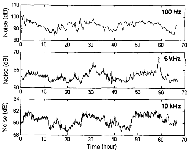
Fig. 5. Variations of ambient noise level about specific frequency band for 70 hours. (a) 100 Hz, (b) 5 kHz, (c) 10 kHz.
