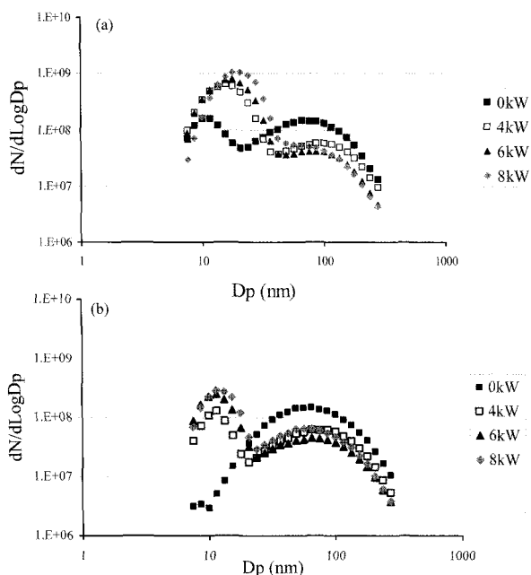
Figure 3. Size distributions of DPM at various engine loads which is doped with (a) 60 ppm Fe and (b) 20 ppm Fe.
