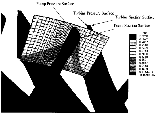
Fig. 9 Pressure distribution according to pump & turbine blade position
