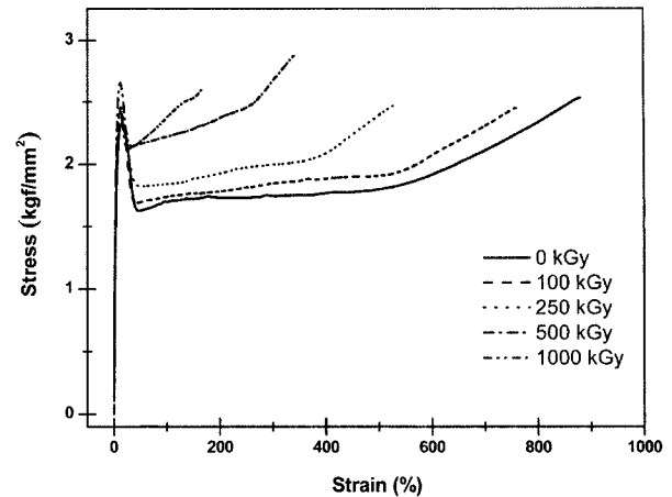
Figure 9. Stress-strain diagrams of irradiated samples.
