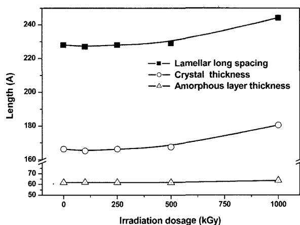
Figure 6. Changes of lamellar long period, crystal thickness and amorphous layer thickness vs. irradiation dosage.
