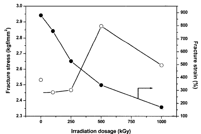
Figure 11. Changes of fracture strain and stress vs. irradiation dosage.
