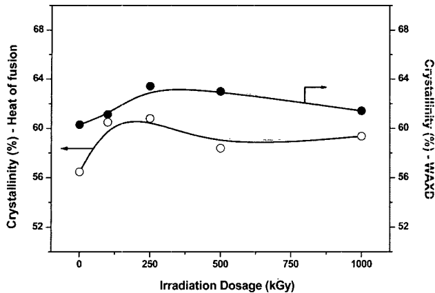
Figure 8. Crystallinities of irradiated samples as determined by wide angle X-ray scattering and DSC.
