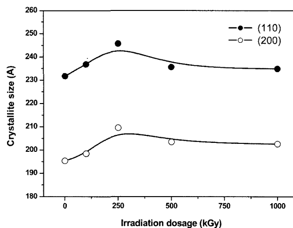
Figure 7. Change of crystal thickness of (110) and (200) planes vs. irradiation dosage.
