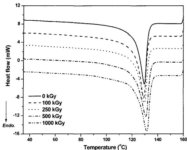
Figure 2. DSC thermograms of electron beam irradiated samples. The curves are arbitrarily shifted.
