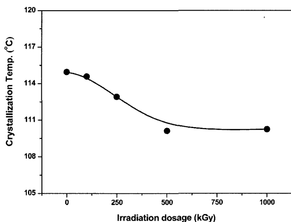
Figure 5. Crystallization temperatures of irradiated samples vs. irradiation dosage.
