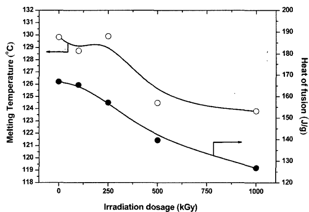
Figure 4. Melting temperature and heat of fusion of irradiated samples after recrystallization.
