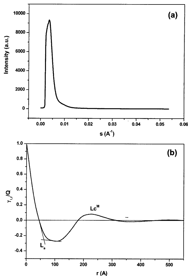
Figure 1. A typical small angle X-ray scattered pattern of lamellar structure (a) and the correlation function derived from the scattered intensities (b).
