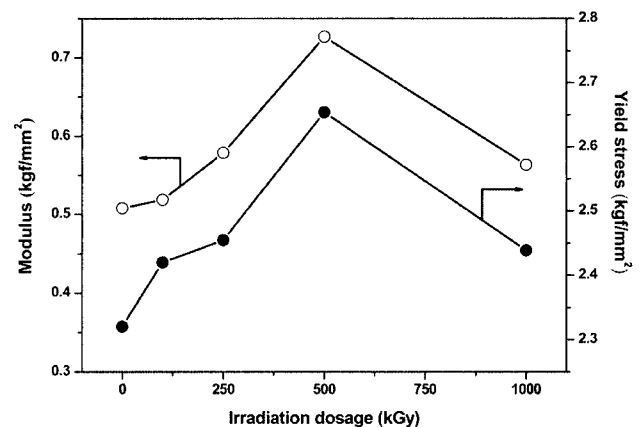
Figure 10. Changes of modulus and yield stress vs. irradiation dosage.
