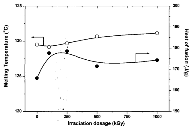
Figure 3. Melting temperature and heat of fusion of irradiated samples at different irradiation dosage.
