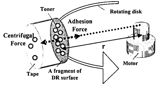
Fig. 6 Centrifugal detachment method
