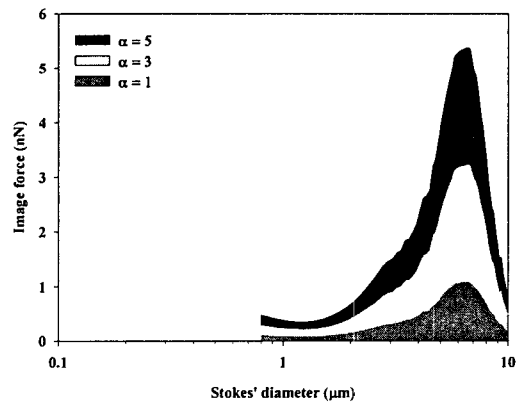
Fig. 7 Image force distribution of charged toner particles
