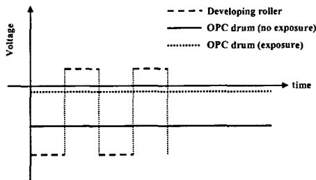
Fig. 2 Operating conditions for developing process
