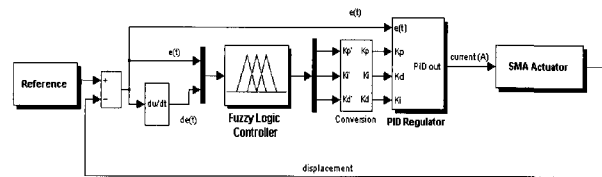
Fig. 11. Schematic diagram of self tuning fuzzy PID controller applied to SMA actuator.
