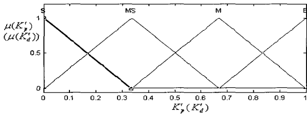
Fig. 5. Membership functions for K_p' and K_d' .
