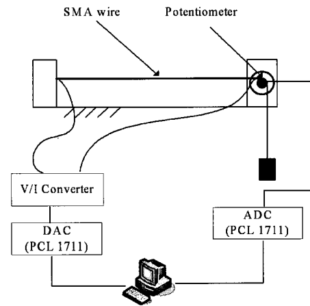
Fig. 10. Experimental apparatus.
