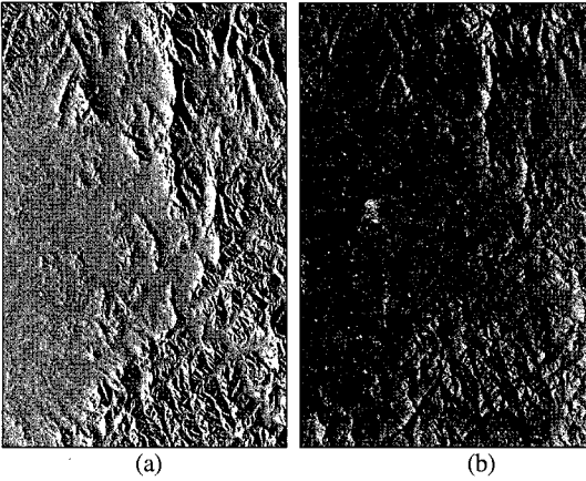
Fig. 2. (a) local incidence angle, (b) corrected image.
