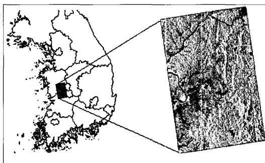
Fig. 1. Study area (Radarsat F5 mode).
