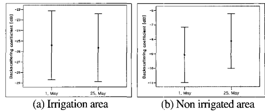
Fig. 3. \sigma^0 variation of agricultural area.
