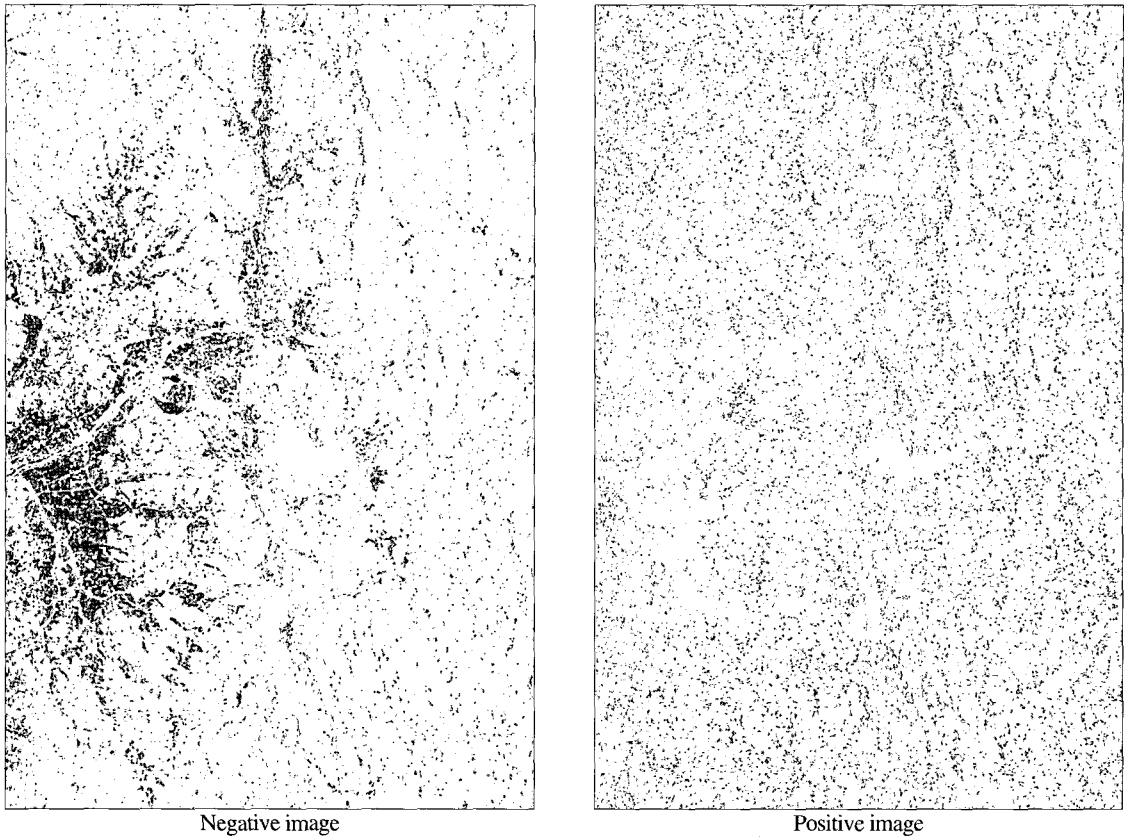
Fig. 4. Change detection differential image (■: large change □: medium change ■: slight change).
