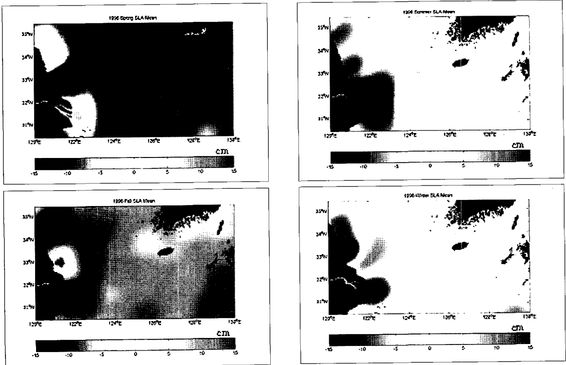
Fig. 2. Seasonal variation in SLAs in 1996.
