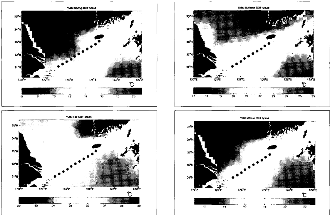
Fig. 3. Seasonal variations in SSTs in 1996.
