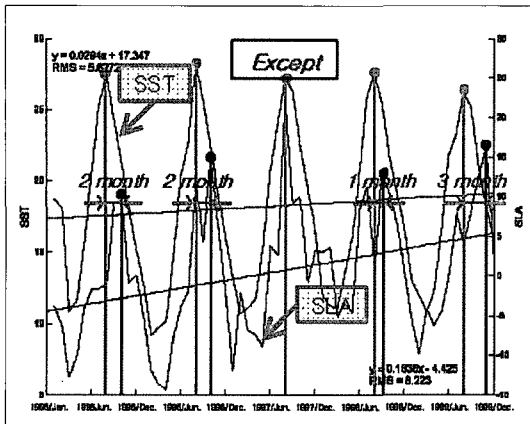
Fig. 5. Time series of SLAs and SSTs in Area A.
