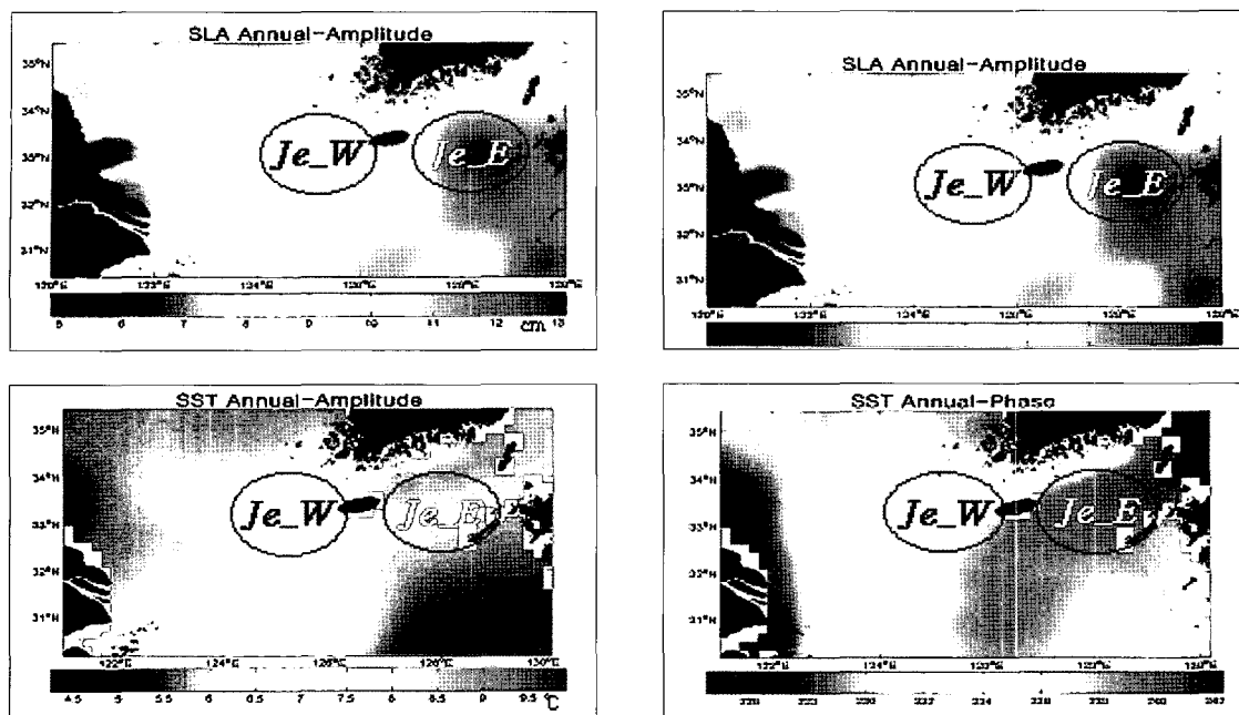
Fig. 4. Harmonic analysis of SLAs and SSTs.
