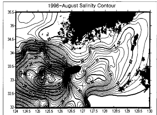
Fig. 6. Distribution of salinity in 1996.
