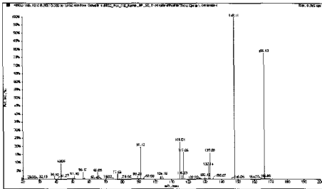
Fig. 3. MS Spectrum of Ephedrine
