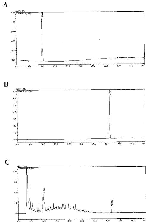
Fig. 1. HPLC Chromatogram of Gamijowitang A: ephedrine, B: schizandrin, C: UV spectra at 210nm of Gamijowitang.
