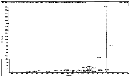
Fig. 4. MS Spectrum of Schizandrin
