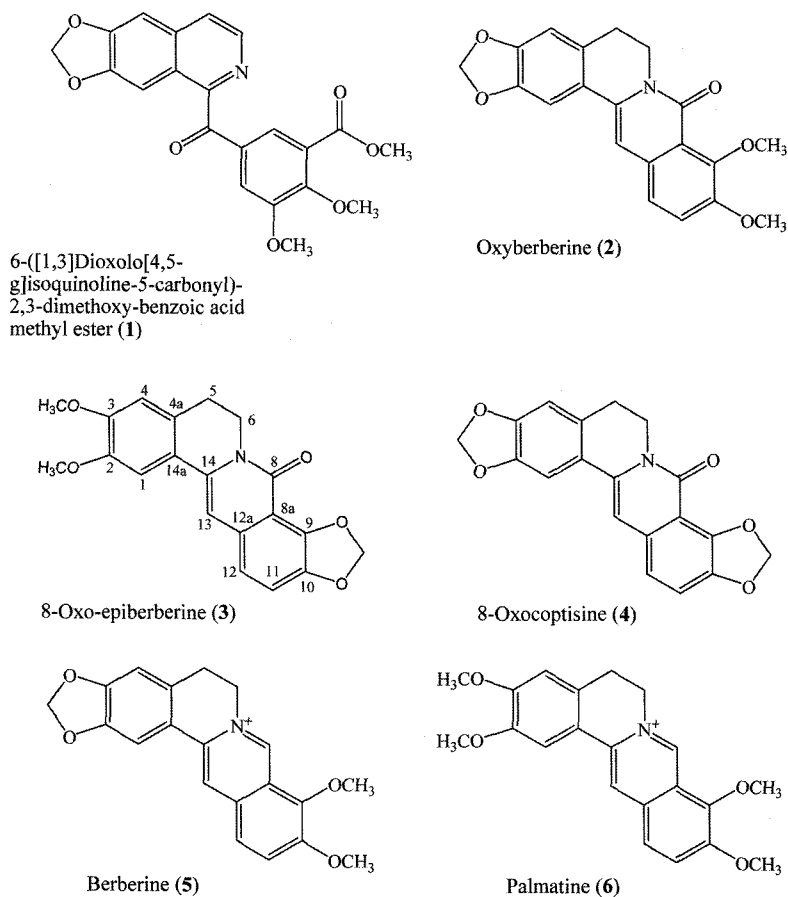
Fig. 1. Structures of compounds 1-6 isolated from C. japonica
