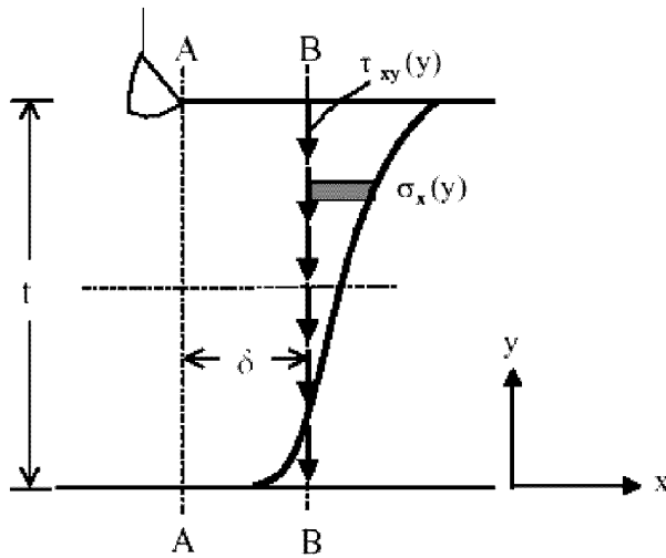
Fig. 2. Structural Stresses Calculation Procedure for Through-Thickness Fatigue Crack
