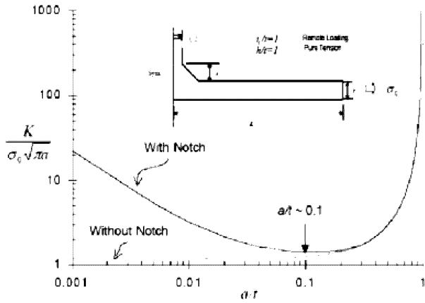
(a) K versus a/t - T joint
