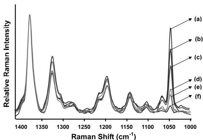
Figure 3. Confocal SERS spectra for varying concentrations of nicotine in the microfluidic channel: (a) 10 ppm, (b) 7.5 ppm, (c) 5.0 ppm, (d) 2.5 ppm, (e) 1.0 ppm, and (f) 0.1 ppm.
