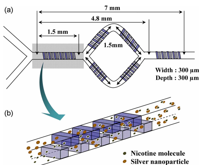
Figure 1. (a) A schematic view of the zig zag-type PDMS microfluidic channel. (b) A mixing process of confluent streams, colloidal silver nanoparticles, and nicotine solution. While laminar flow streams traverse the microfluidic channel, the transverse and vertical dispersion of the fluid occurs simultaneously through the upper and lower blocks.
