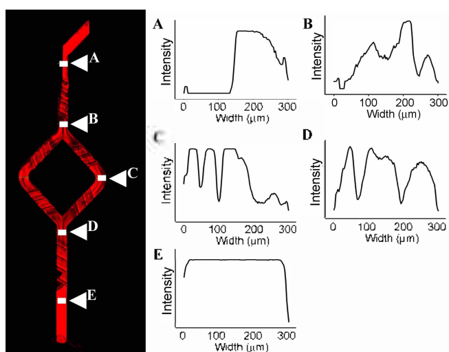
Figure 2. Confocal fluorescence images of lateral confluent streams along the channel and corresponding intensity profiles at the locations indicated by the solid lines.
