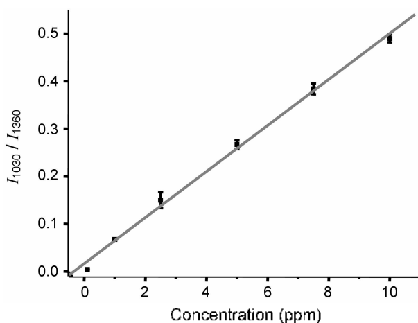
Figure 4. Variation of the peak area ratio ( I_{1030}/I_{1360} ) as a function of nicotine concentration. (Correlation coefficient, R = 0.998 )
