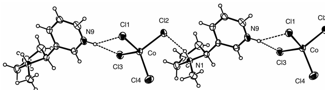
Figure 3. A view of hydrogen-bonding mode between nicotinium cation and CuCl 4 2- anion showing selected atom labels.
