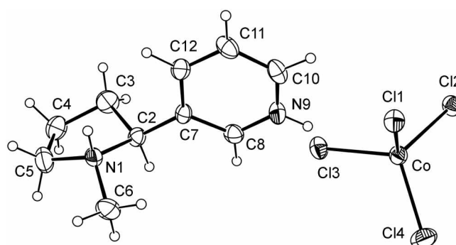
Figure 2. ORTEP diagram of (nicH 2 )CoCl 4 , showing the atom numbering scheme.
