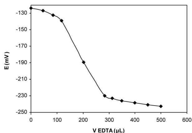
Figure 5. Potentiometric titration curve of 20.0 mL 1.0 × 10 -6 M solution of Cu 2+ with 1.0 × 10 -4 M of EDTA.
