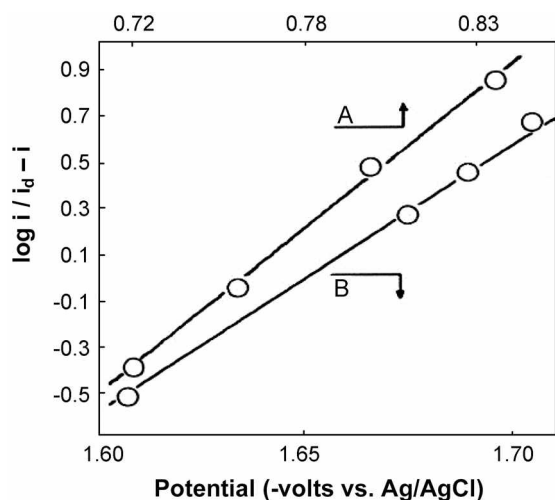
Figure 4. A plot of \log i / (i_d - i) vs. potential for polarograms on the 1 \times 10^{-3} M ABMC. A: 1st wave: slope 84 mV, B: 2nd wave: slope 73 mV, *: 3rd wave: poor DC polarogram to plot.
