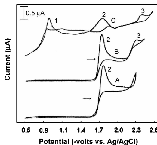
Figure 3. Typical cyclic voltammograms of coumarin derivatives in 0.1 M TEAP-AN solution. Scan rate: 50 mV/sec. A: 1 \times 10^{-3} M coumarin, B: 1 \times 10^{-3} M AMC, C: 5 \times 10^{-4} M ABMC.
