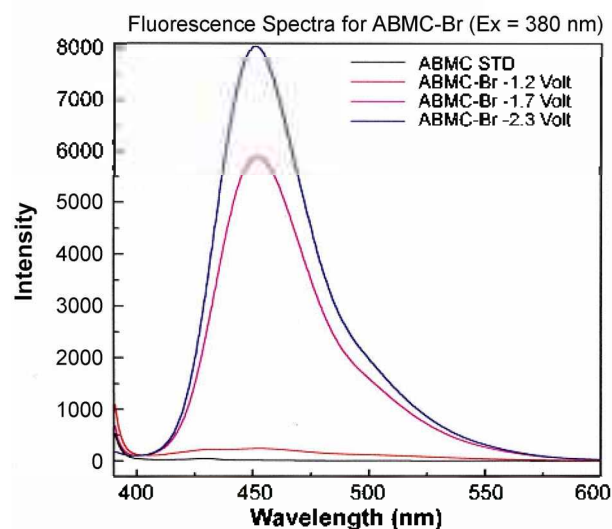
Figure 9. Fluorescence spectra for the ABMC depend on the controlled potential of electrolysis.
