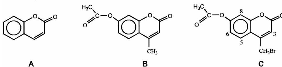
Figure 1. Structure of A: coumarin, B: 7-acetoxy-4-methyl-coumarin (AMC), C: 7-acetoxy-4-bromomethyl-coumarin (ABMC).
