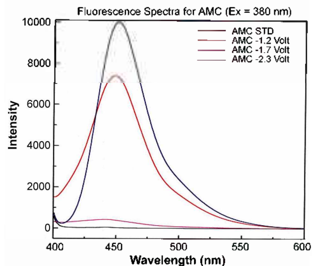
Figure 8. Fluorescence spectra for the AMC depend on the controlled potential of electrolysis.
