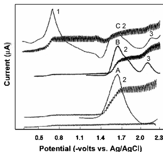
Figure 2. Typical DC and DP polarograms of coumarin derivatives in 0.1 M TEAP-AN solution. Scan rate: 50 mV/sec. Current range: 0.02 mA. A: 1 \times 10^{-3} M coumarin, B: 1 \times 10^{-3} M AMC, C: 5 \times 10^{-4} M ABMC.
