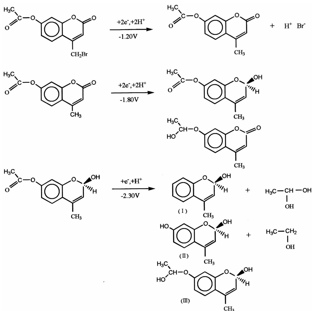
Scheme 1. The proposed electrochemical reduction mechanism on the ABMC.
