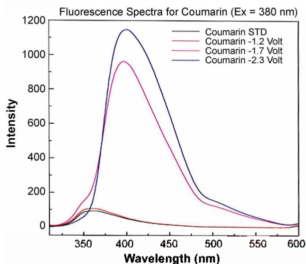
Figure 7. Fluorescence spectra for the coumarin basic molecule depend on the controlled potential of electrolysis.
