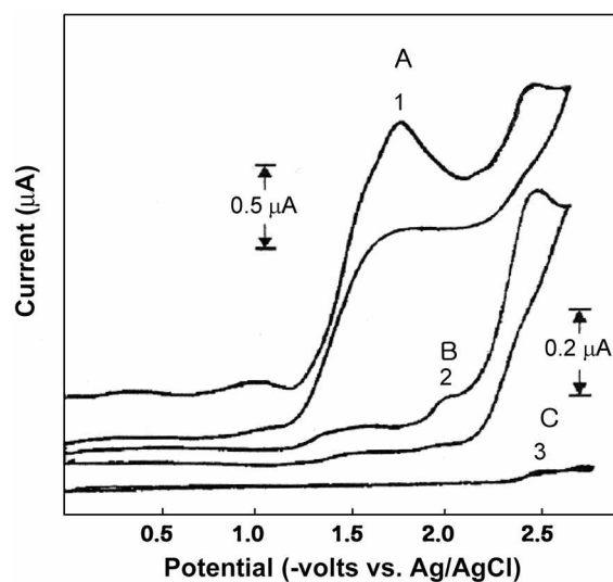
Figure 6. Cyclic voltammograms of electrolyzed solution for ABMC. A: after 1st step electrolysis at -1.2 volts, B: after 2nd step electrolysis at -1.8 volts, C: after 3rd electrolysis at -2.3 volts.
