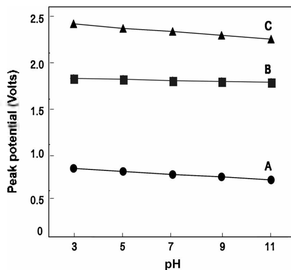
Figure 5. Effect of pH change in peak potentials of 1 \times 10^{-3} M ABMC in 0.1 M TEAP-AN solution. ● : 1st wave ■ : 2nd wave ▲ : 3rd wave.
