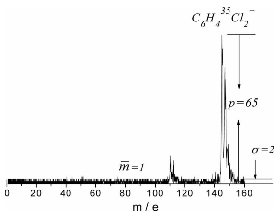
Figure 7. Mass spectrum of 1,4-DCB at 248 nm (the concentration is 2 ppm, \epsilon=2 ppm).
