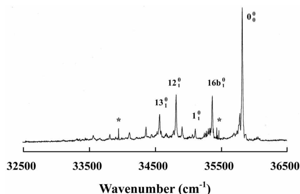
Figure 1. A portion of the vibronic emission spectrum of the jet-cooled m -tolunitrile in the S_1 \rightarrow S_0 transition recorded with a FT spectrometer. The molecules were vibrationally excited in a corona-excited supersonic expansion using a pinhole-type glass nozzle. The peaks marked with an asterisk in this spectrum indicate the He atomic transitions.
