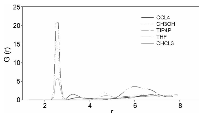
Figure 2. Radial distribution functions g(r) , of 18-crown-6/ \text{Nd}^{3+} ion complex in selected solvents. Distances are in angstroms throughout.
