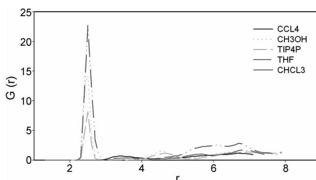
Figure 3. Radial distributions functions of 18-crown-6/ \text{Eu}^{3+} ion complex in selected solvents.
