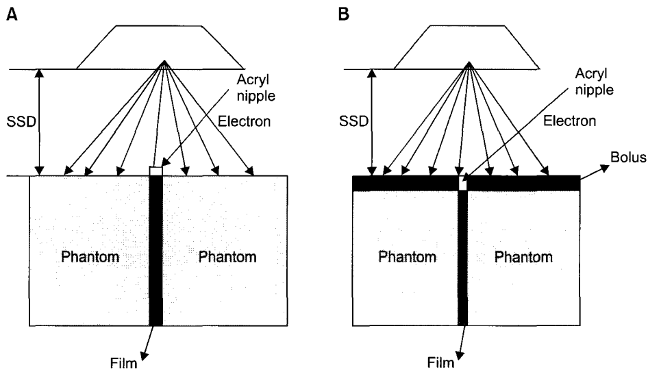
[Fig. 2] The Nipple and bolus experimental setup, (A) non bolus setup, (B) use of bolus setup
