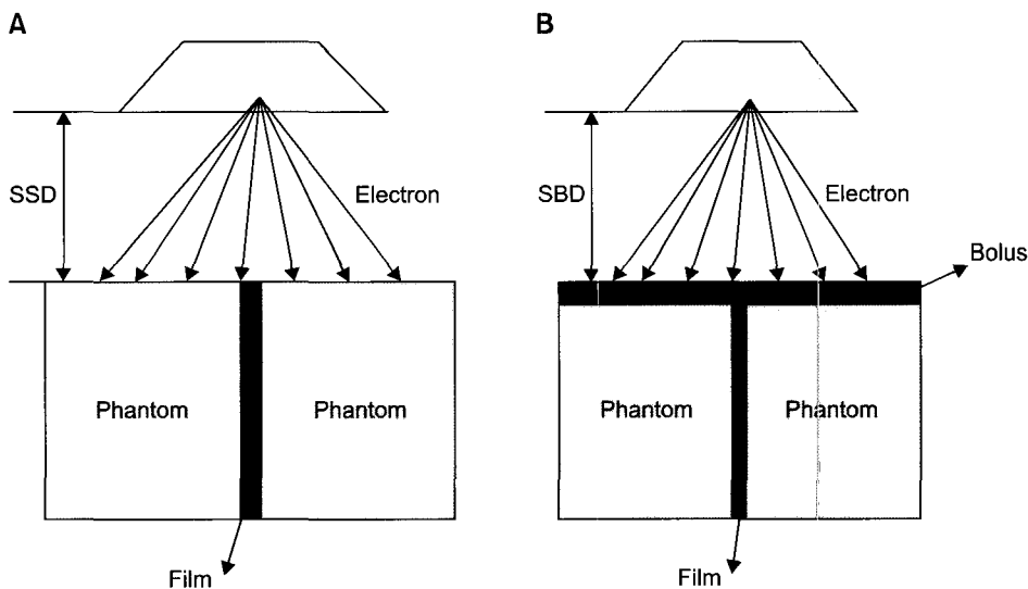
[Fig. 1] The SSD and SBD experimental setup, (A) SSD setup, (B) SBD setup
