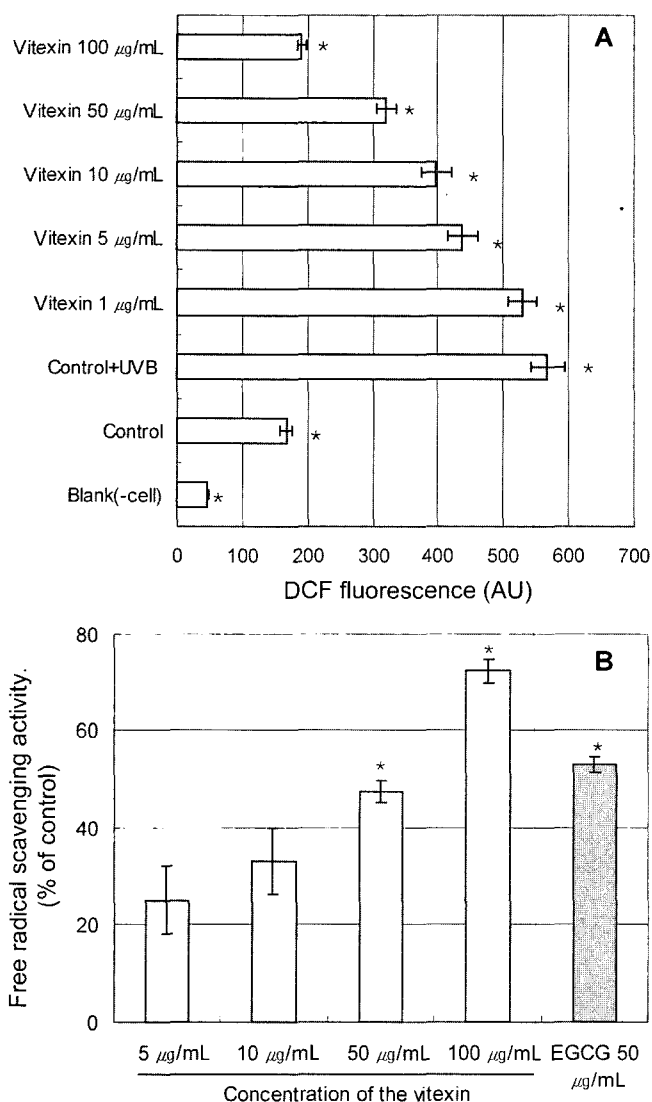
Fig. 4. A: The effects of vitexin on the production of intracellular reactive oxygen species (ROS) in human dermal fibroblasts (HDFs). HDFs were incubated with 4 \mu\text{M} CM-H 2 DCFDA for 20 min, and irradiated by UVB 20 mJ/cm 2 . Various concentrations of vitexin were used for treatment. ROS generation was assessed by luminescence spectrophotometer. The values of DCF fluorescence are significant (* p <0.05). Values are expressed as mean \pm S.E.M. B: Free radical scavenging activity after UV irradiation in human dermal fibroblasts (HDFs). ROS generation was assessed by luminescence spectrophotometer. Vitexin ( \square ) reduced the UVB-induced fluorescence increase in a dose dependent manner. EGCG ( \blacksquare ) was used as a positive control. The values of DCF fluorescence are significant (* p <0.05). Values are expressed as mean \pm S.E.M.
