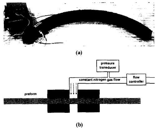
Fig. 4 Preform test prior to insertion into mold: (a)experimental setup; (b) schematic of measurement[18].
