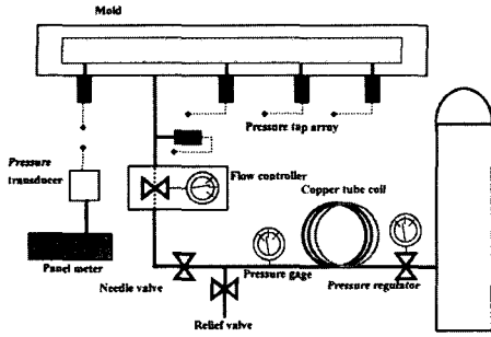
Fig. 1 Overall view of experimental setup[10].
