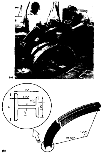
Fig. 3 (a) Assemblage of mold prior to test; (b) shape and dimension of mold cavity[18].
