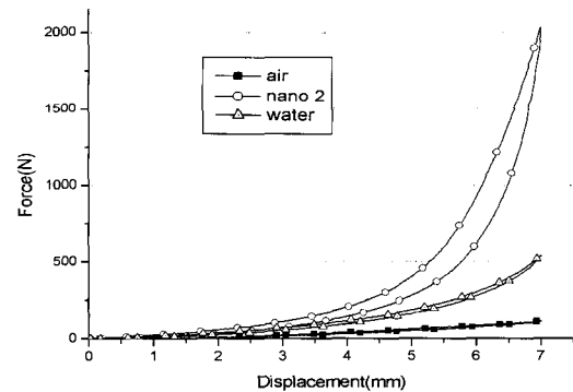
Fig. 10 Force-displacement curve of each pocket for 7 mm displacement
