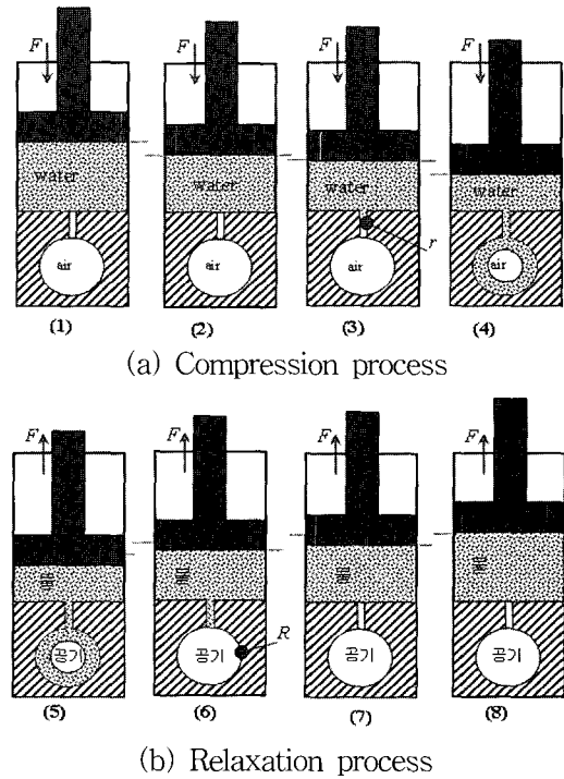
Fig. 3 Process of energy dissipate cycle model
