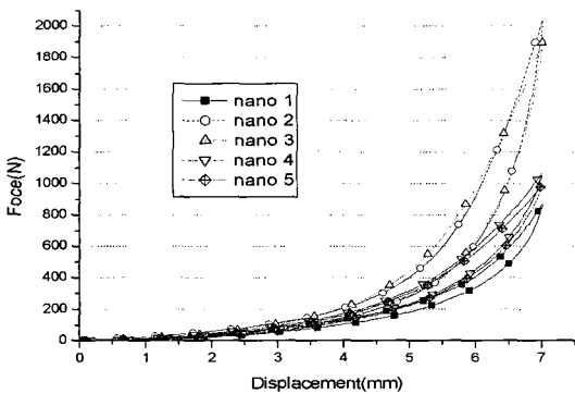
Fig. 7 Force-displacement curve of each pocket for 7 mm displacement
