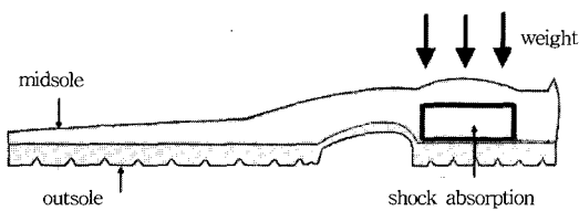
(b) Mid. outsole and of shock
