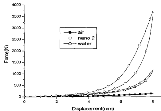
Fig. 11 Force-displacement curve of each pocket for 8 mm displacement
