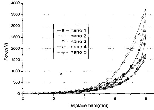
Fig. 8 Force-displacement curve of each pocket for 8 mm displacement
