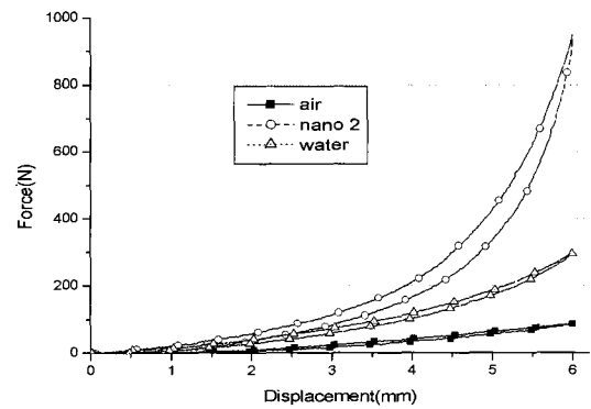
Fig. 9 Force-displacement curve of each pocket for 6 mm displacement
