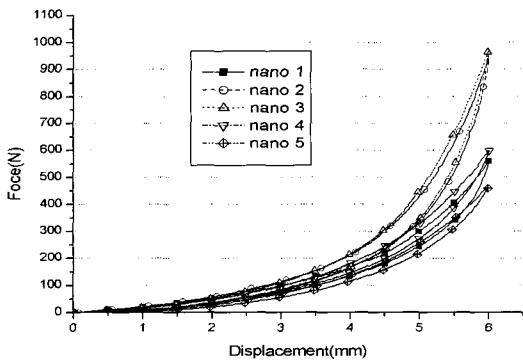
Fig. 6 Force-displacement curve of each pocket for 6 mm displacement
