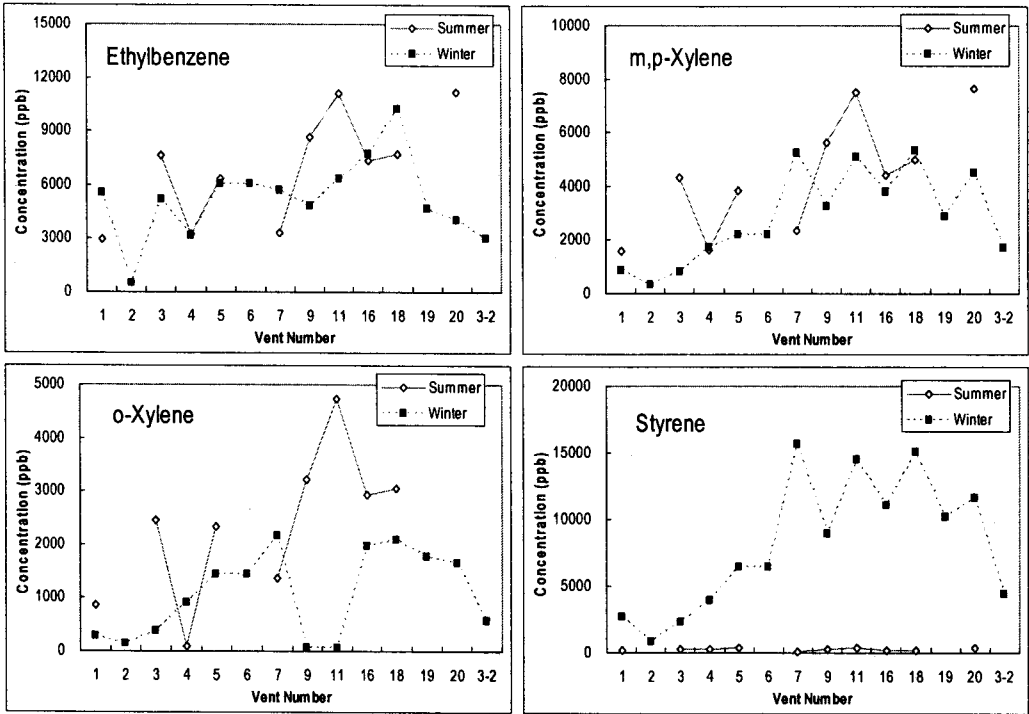
〈그림 4〉 Comparison of major aromatic VOC in LFG samples, collected from the new landfill site in Donghae, is made as a function of vent number.
