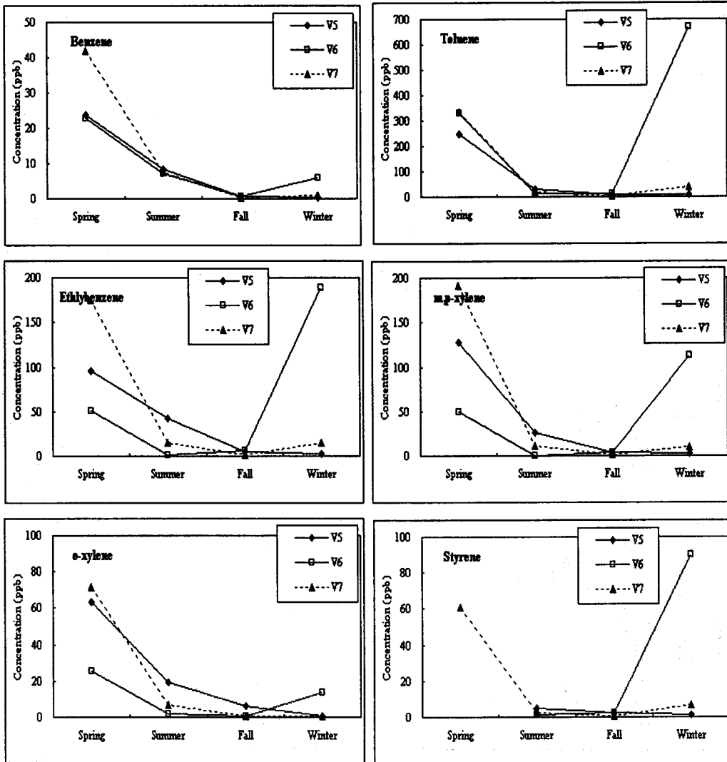
<그림 5> Comparison of major aromatic VOC in LFG samples, collected from the old landfill site in Donghae, is made as a function of vent number.
