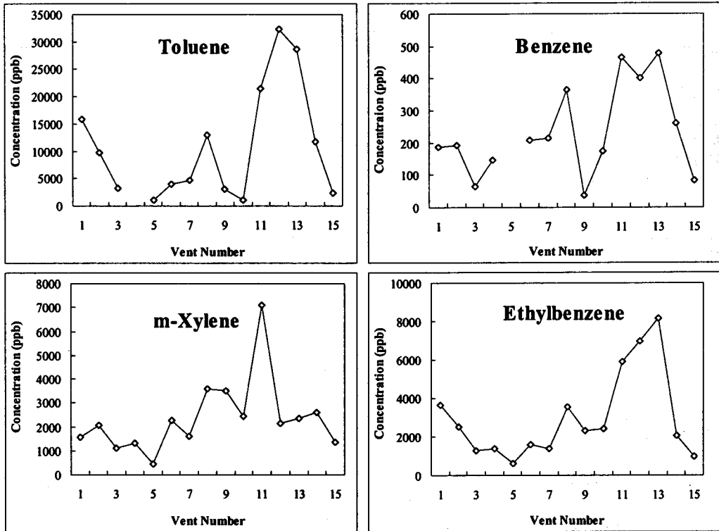
<그림 2> The LFG concentration of major aromatic VOC determined from the WJ site during winter 2002 period are compared as a function of vent number.
