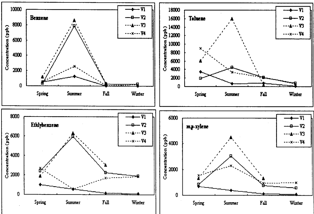
〈그림 4〉 Comparison of major aromatic VOC in LFG samples, collected from the new landfill site in Donghae, is made as a function of vent number.
