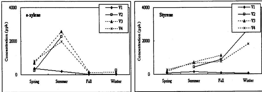
<그림 5> Comparison of major aromatic VOC in LFG samples, collected from the old landfill site in Donghae, is made as a function of vent number.
