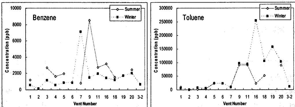
<그림 3> The LFG concentration of major aromatic VOC determined from the BC site between winter(Jan) and summer(Aug.) 2004 period are compared as a function of vent number.
