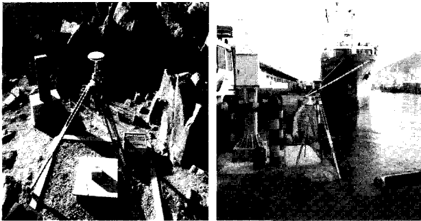
Fig. 5 Image of GPS static surveying performance
