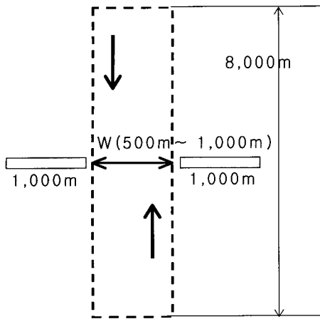
Fig. 1 Area Condition of Marine Traffic Simulation
