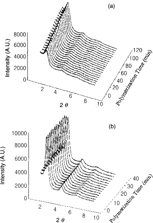
Figure 3. Real-time X-ray diffraction patterns for (a) 10A-MMT/PS and (b) 15A-MMT/PS, polymerized in-situ at 60 °C.
