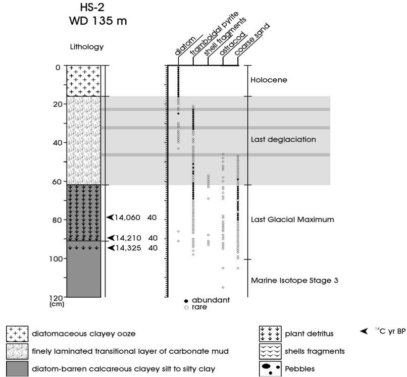
Fig. 2. Lithology, water content, sand fractions, and constituent compositions in core HS-2 from Lake Hovsgol.
