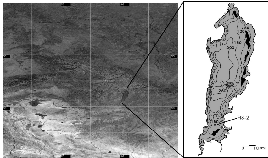
(from Image Science and Analysis Laboratory, NASA-Johnson Space Center). Fig. 1. Location map of Lake Hovsgol in northern Mongolia.
