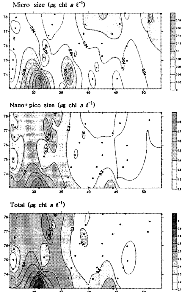
Fig. 6. Contour of surface chlorophyll-a(biomass) concentrations.
