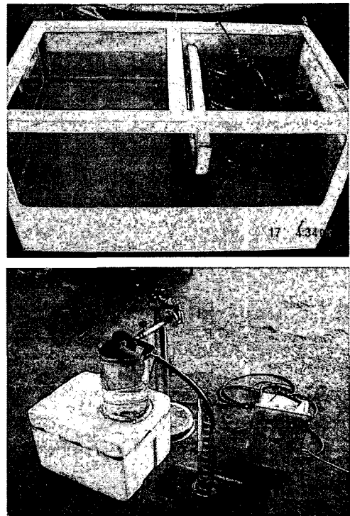
Fig. 2 The experimental apparatus, measuring water tank for mass of recovery oil and measuring device for recovery rate of pure oil and water.
