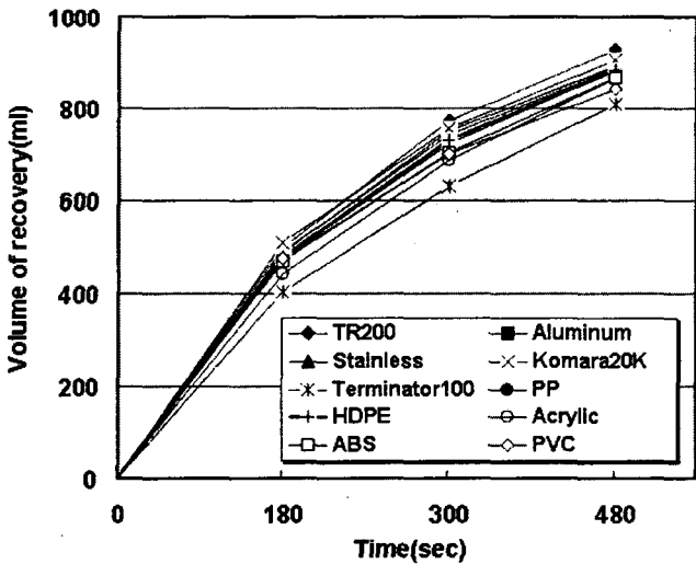
Fig. 3 Variations of volume of bunker A oil recovered by experimental disks with times.
