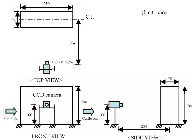
Figure 1. Dimensional sketch of the system for recognizing individual cattle.
