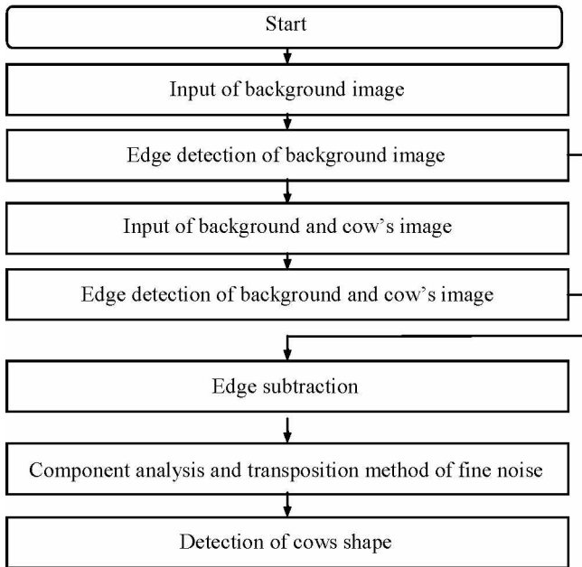
Figure 3. Flowchart of pre-processing for shape detection.
