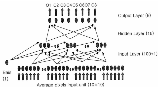
Figure 8. Structure of neural network learning for pattern recognition.
