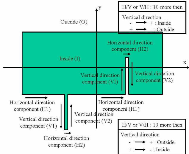
Figure 4. Thinning transferring method for noise reduction.
