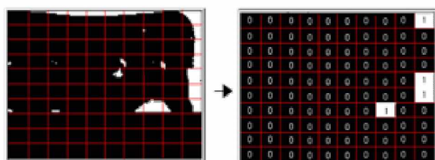
Figure 7. Input binary values in the neural network.
