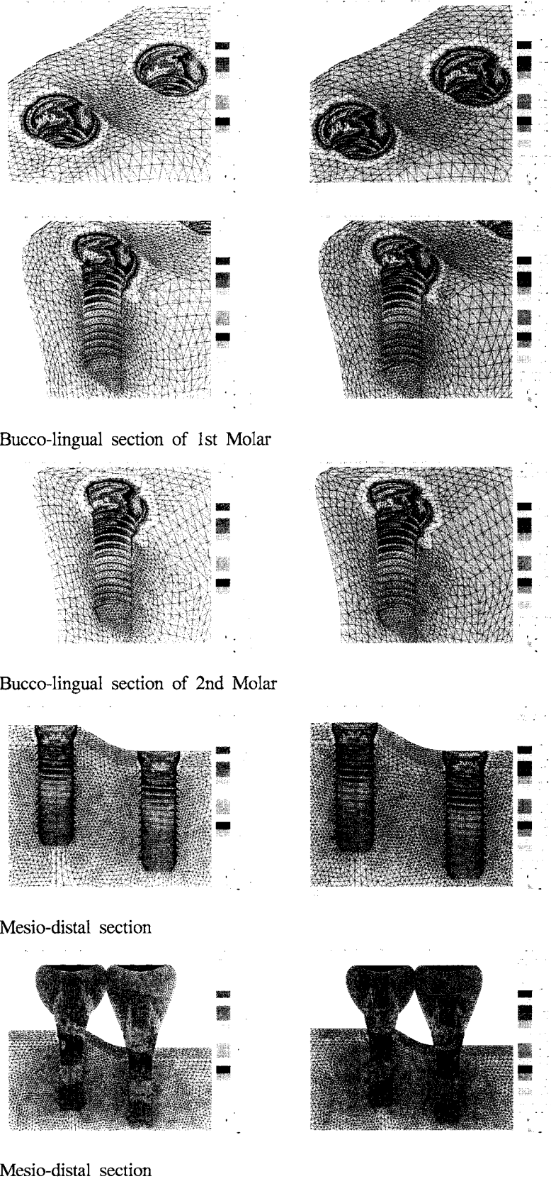
Fig. 9. The von Mises stress value on the bucco-lingual and mesio-distal sections under vertical loading condition C (Left side: Model 1, Right side: Model 2).
