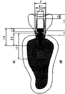
Fig. 2. The bucco-lingual section of the full body (unit: mm).
