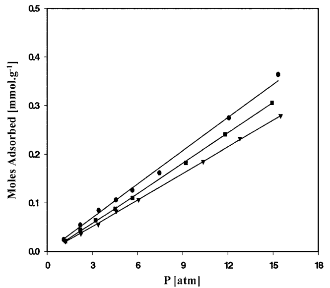
Fig. 5. Adsorption equilibrium curve of H 2 ; ▼, 293.15 K; ■, 303.15 K; ◆, 313.15K; —, LRC model.
