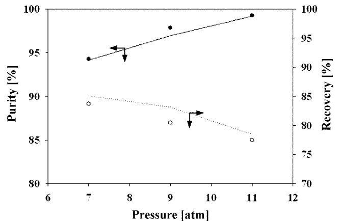
Fig. 11. Effect of adsorption pressure at 22 LPM flowrate and 0.10 P/F ratio, ●; experiment, —; simulation.
