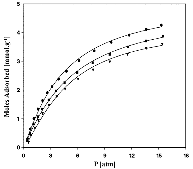
Fig. 4. Adsorption equilibrium curve of CH 4 ; ▼, 293.15 K; ■, 303.15 K; ◆, 313.15 K; —, LRC model.
