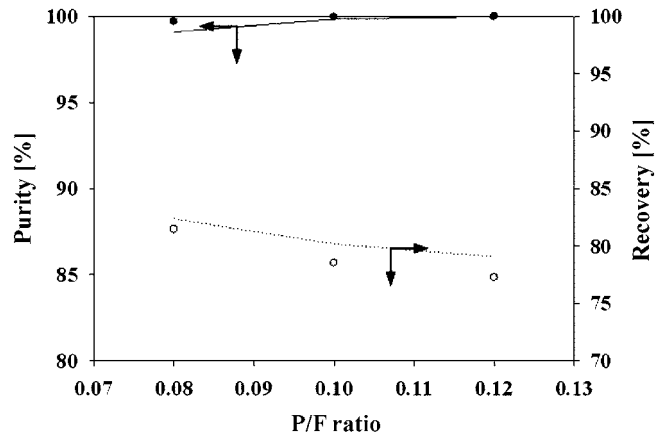
Fig. 10. Effect of P/F ratio at 22 LPM flowrate and 11 atm pressure, ●; experiment, —; simulation.
