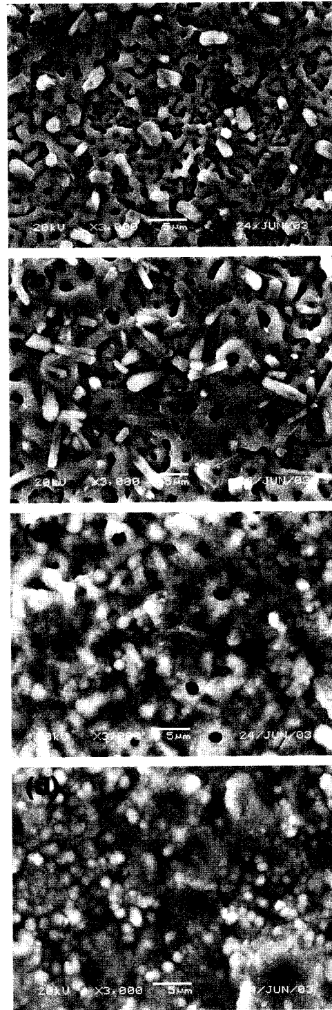
Fig. 4. Scanning electron micrographs of anodized at (a) 240 V, (b) 280 V, (c) 320 V, and (d) 360 V following hydrothermally treated at 300°C for 2 hrs and immersed in Hanks' solution for 30 days.
