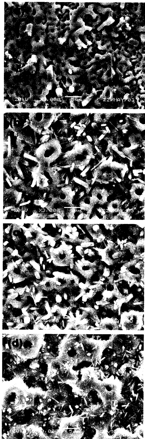
Fig. 2. Scanning electron micrographs of anodized at (a) 240 V, (b) 280 V, (c) 320 V, and (d) 360 V following hydrothermally treated at 300°C for 2 hrs.
