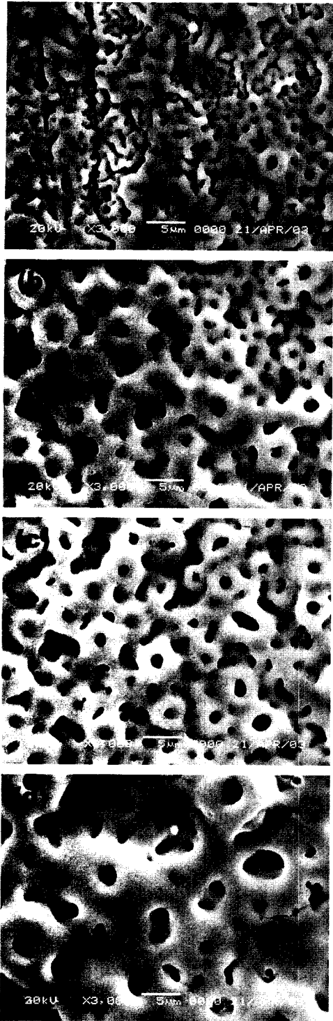
Fig. 1. Scanning electron micrographs of anodic oxide films formed at (a) 240, (b) 280, (c) 320, and (d) 360 V.
