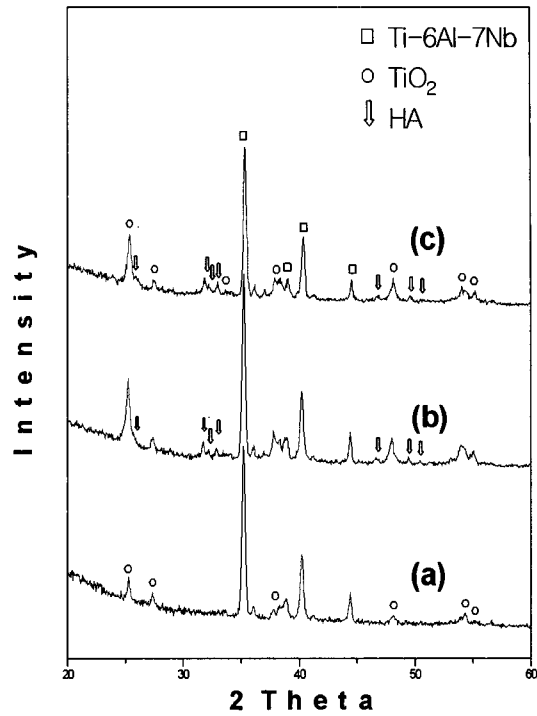
Fig. 6. XRD patterns of each steps in 360V. (a) anodized, (b) hydrothermally treated for 2 hrs, (c) immersed in Hanks' solution for 30 days.
