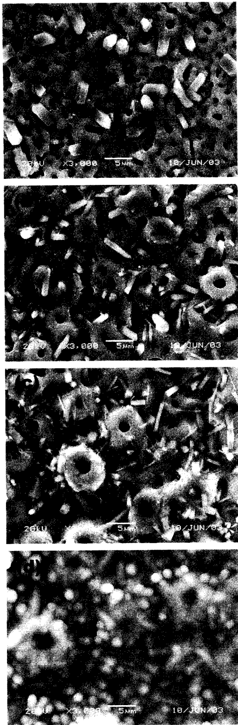
Fig. 3. Scanning electron micrographs of anodized at (a) 240 V, (b) 280 V, (c) 320 V, and (d) 360 V following hydrothermally treated at 300°C for 2 hrs and immersed in Hanks' solution for 15 days.
