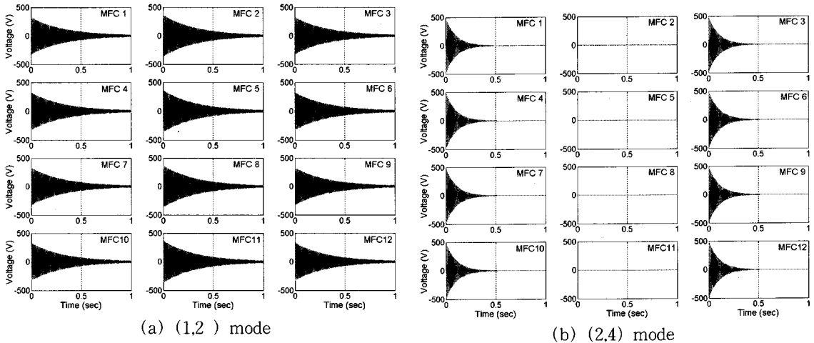
Fig. 12 Voltage history of each actuator
