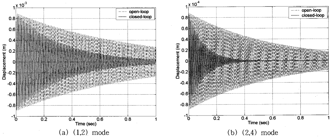
Fig. 11 Open-loop and closed-loop transient response under (1,2) mode and (2,4) mode motion
