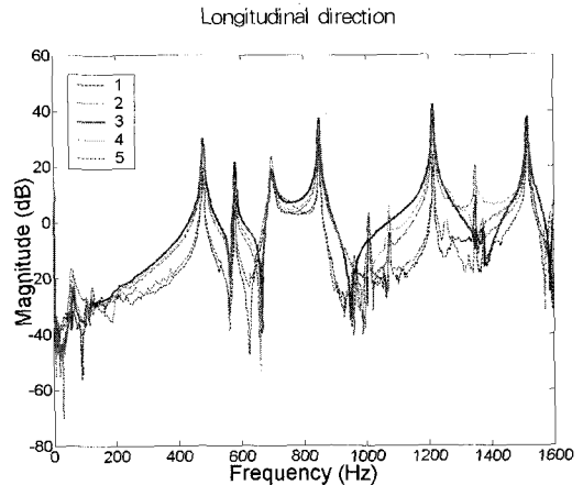
Fig. 10 System response of hull structure along length direction
