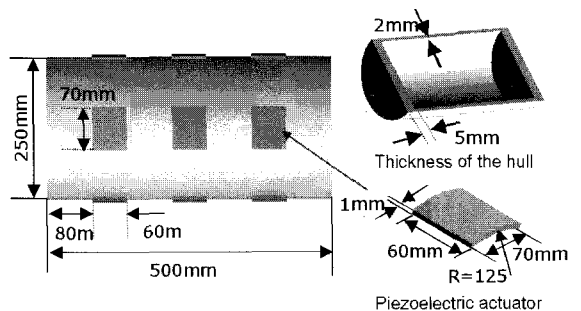
Fig. 6 Geometry of the end-capped hull structure with surface bonded MFC actuators
