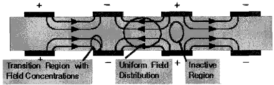
Fig. 2 Electric field distribution for interdigitated electrode (16)
