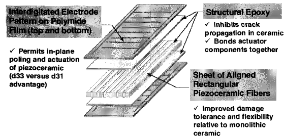
Fig. 1 Schematic diagram of macro fiber composite actuator (11)
