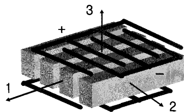
(a) Electrodes of MFC actuator
