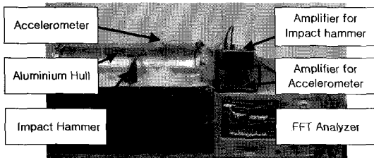
Fig. 9 Experimental setup for modal test
