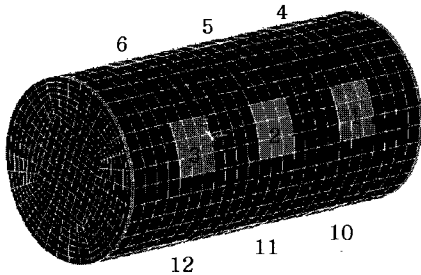
Fig. 7 Finite element mesh configuration
