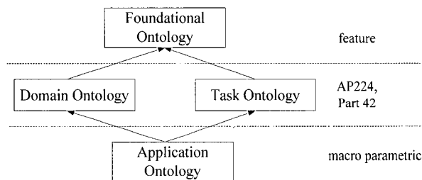
Figure 1: Layered ontology
