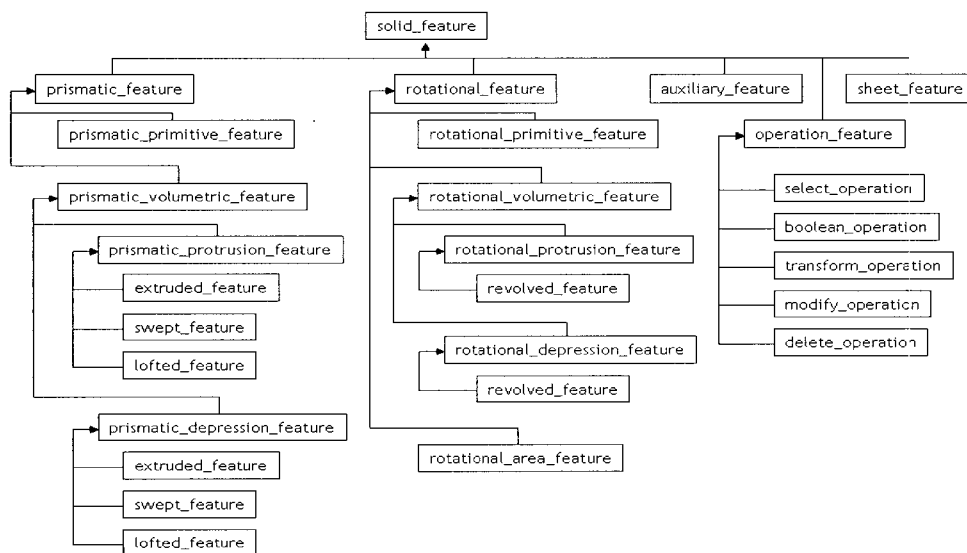
Figure 3: Feature taxonomy
