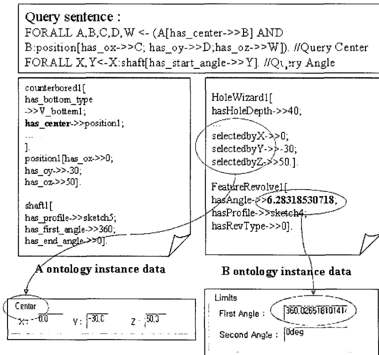
A system view with B ontology data
