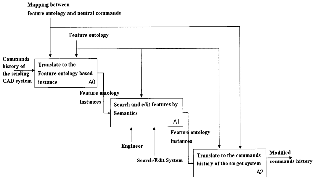
Figure 8: IDEF0 diagram of the implemented system
