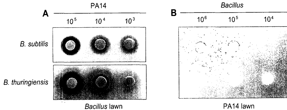
Fig. 2. Interaction between P. aeruginosa and Bacillus spp. (A) The Bacillus plate killing assay was done with serially-diluted PA14 culture suspensions spotted on either B. subtilis (upper) or B. thuringiensis (lower) lawns. The numbers ( 10^5 , 10^4 , and 10^3 ) indicate the CFU in the PA14 cell spots. (B) A reversed plate killing assay was done with serially-diluted B. subtilis (upper) and B. thuringiensis (lower) culture suspensions spotted on the PA14 lawn. The numbers ( 10^6 , 10^5 , and 10^4 ) indicate the CFU in the Bacillus cell spots.
