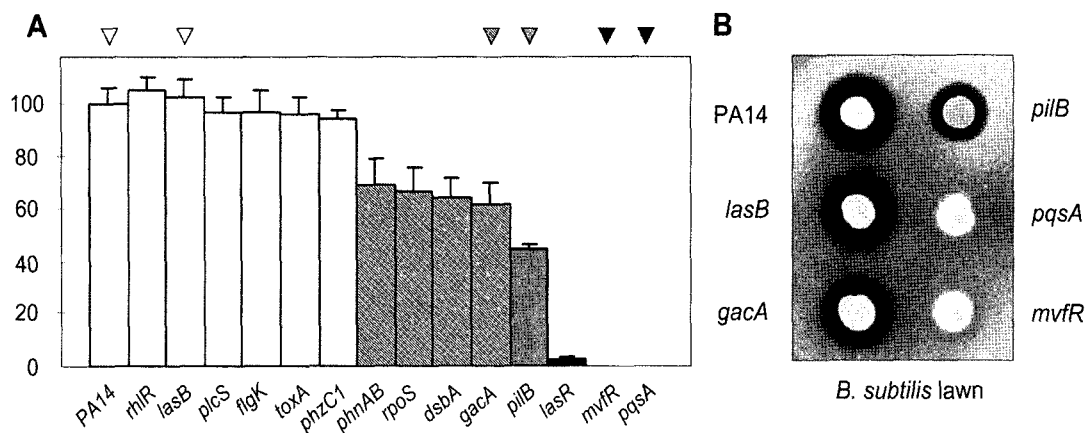
Fig. 4. Involvement of virulence factors in B. subtilis killing. (A) The B. subtilis killing indices of the PA14 mutants are represented as the relative value to the size of the PA14-derived halo (see Materials and Methods). The size of the halos was measured in five independent experiments. Based on these indices, P. aeruginosa strains and PA14 mutants were classified into four groups: group 1 (empty bar), highly killing (PA14, rhIR , lasB , plcS , flgK , toxA , and phzC1 ); group 2 (stripe bar), moderately killing ( phnAB , rpoS , dsbA , and gacA ); group 3 (gray bar), slightly killing ( pilB ); group 4 (black bar), unkillable ( lasR , mvfR , and pqsA ). The values indicate the averages of five independent experiments with the error bars representing standard deviations. (B) Several PA14 mutants (arrowheads in A) representing each group were subjected to the Bacillus plate killing assays on LB media. lasB (group 1), gacA (group 2), pilB (group 3), mvfR , and pqsA (group 4) mutants were included, with PA14 as the control.
