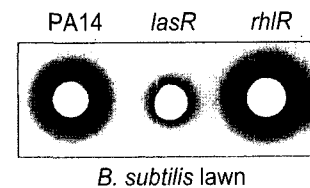
Fig. 3. Involvement of N -acyl-L-homoserine lactone (AHL)-dependent quorum sensing (QS) systems in B. subtilis killing. The Bacillus plate killing assay was performed on an LB plate using the PA14 mutants defective in AHL-dependent QS systems ( lasR and rhlR ), as in Fig. 1.
