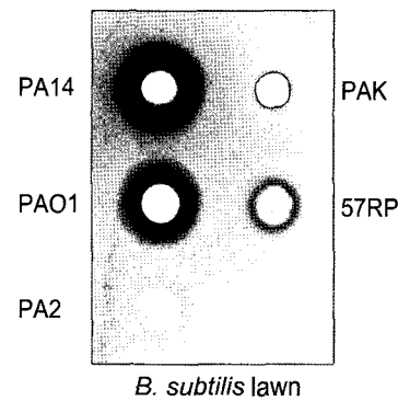
Fig. 1. Visualization of the P. aeruginosa - B. subtilis interaction. The Bacillus plate killing assay was performed on an LB plate, using P. aeruginosa strains (PA14, PAO1, PAK, 57RP, and PA2) as described in Materials and Methods.
