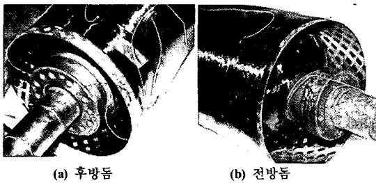
Fig. 6 Ingress/egress of FBG sensor lines for STEB2.
