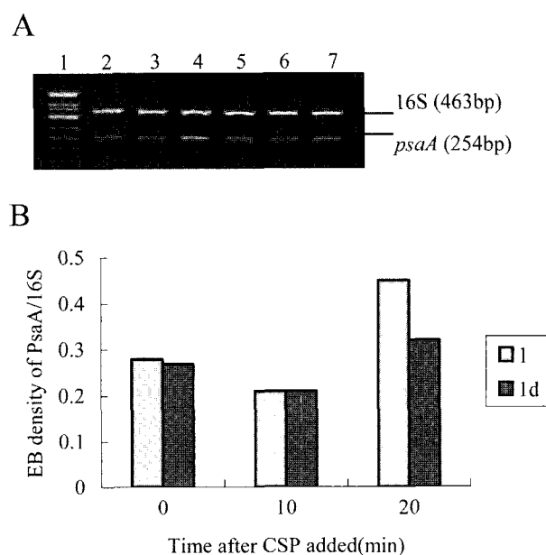
Fig. 3. (A) RT-PCR psaA of S. pneumoniae strains 1 and 1d on 2% agarose gel electrophoresis. Lane 1, Marker2; lanes 2-4, 0 min, 10 min, 20 min after CSP was added into S. pneumoniae No.1; lanes 5-7: 0 min, 10 min, 20 min after the addition of CSP to S. pneumoniae strain 1d. (B) psaA mRNA expression of S. pneumoniae strains 1 and 1d, at different times. psaA mRNA expression was compared with that of 16S rRNA after the addition of CSP to bacteria at 0 min, 10 min or 20 min timepoints in strains 1 and 1d, using Quantity-one software.
