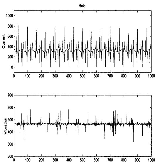
Fig. 8. Measured sensor signals of the holed bearing
