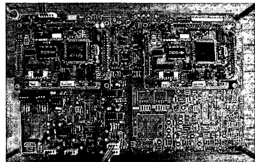
Fig. 4 View of redundancy system
