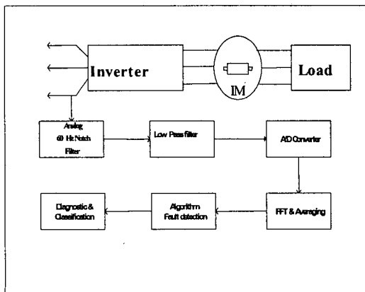
Fig. 2. Block diagram of single phase stator current monitoring scheme
