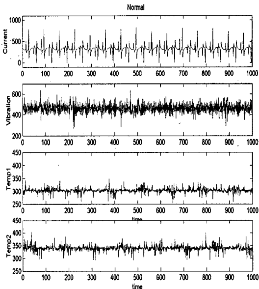
Fig. 7. Measured sensor signals of normal condition motor
