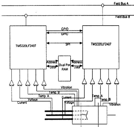
Fig. 1. Block diagram of redundancy system
