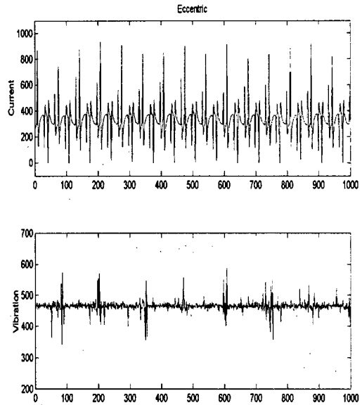
Fig. 9. Measured sensor signals of the eccentric motor shaft
