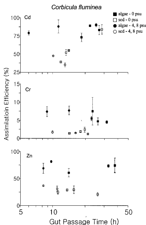
Fig. 2. Relationships of metal assimilation efficiencies (AEs; %) with gut passage time (GPT; hr) of Cd, Cr and Zn in Corbicula fluminea fed algal or sediment particles under varying salinity and temperature levels.
