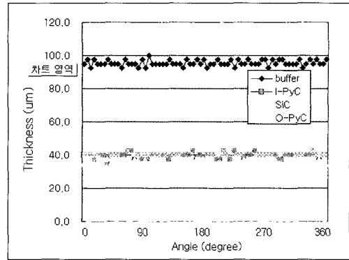
Fig. 11. Measured coating thickness
