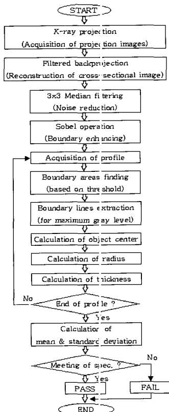
Fig. 6. Automatic measurement algorithm for the coating thickness
