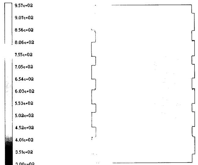
Fig. 4. Planar view of temperature distribution of 10th separator (6 kW, U_f=U_o=0.6 , i=150 mA/cm 2 ).
