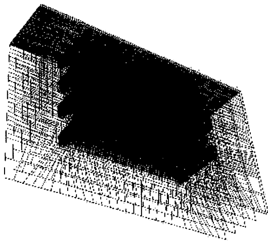
Fig. 2. 6 kW-class stack grid.
