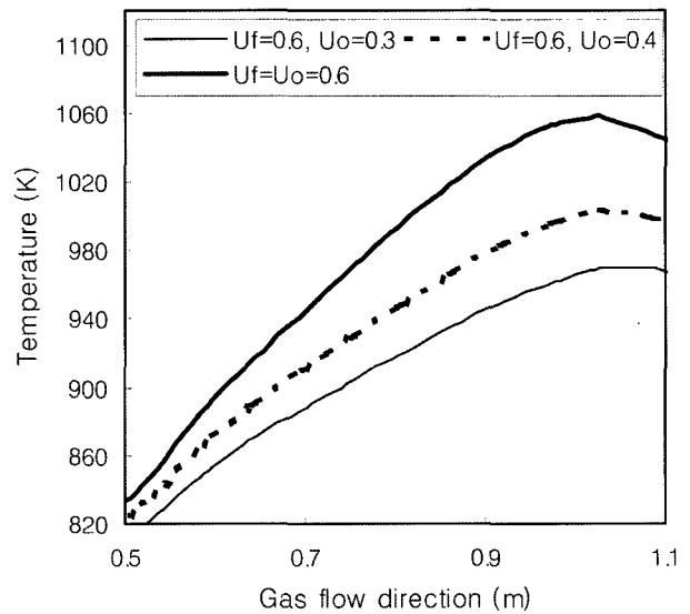
Fig. 11. Temperature of 10th separator of 25 kW stack at different air utilization rate ( U_f=0.6 , i=150 \text{ mA/cm}^2 ).
