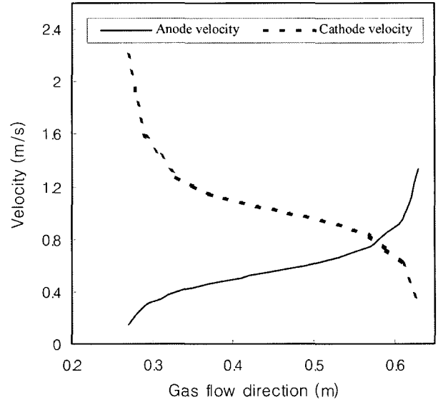
Fig. 10. Velocity distribution of 10th channel (6 kW, U_f=U_o=0.6 , i=150 \text{ mA/cm}^2 ).
