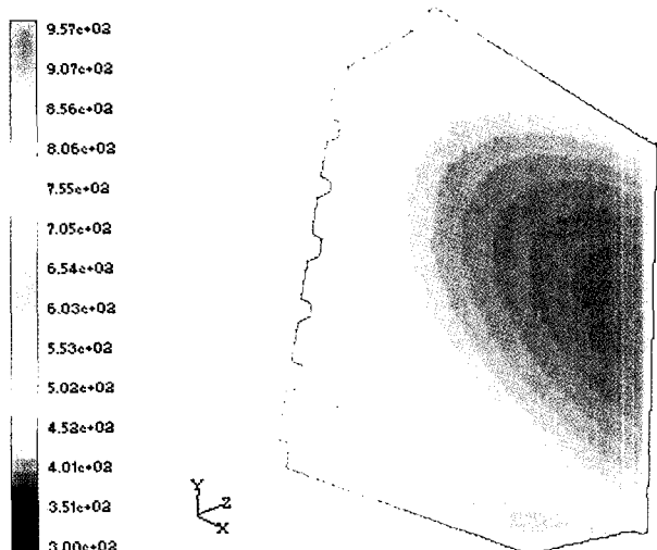
Fig. 5. Planar view of temperature distribution of MCFC stack (6 kW, U_F=U_o=0.6 , i=150 mA/cm 2 ).
