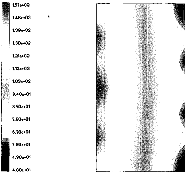
Fig. 9. Planar view of pressure distribution of 10th cathode channel (6 kW, U_f=U_o=0.6 , i=150 \text{ mA/cm}^2 ).
