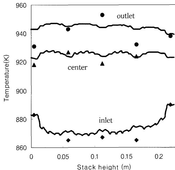
Fig. 7. Temperature distributions compared with experimental data (6 kW, U_F=U_o=0.6 , i=150 mA/cm 2 ).
