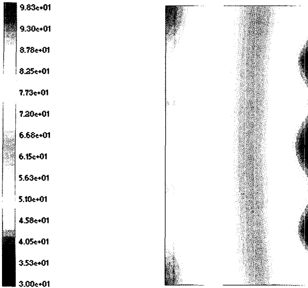
Fig. 8. Planar view of pressure distribution of 10th anode channel (6 kW, U_f=U_o=0.6 , i=150 \text{ mA/cm}^2 ).
