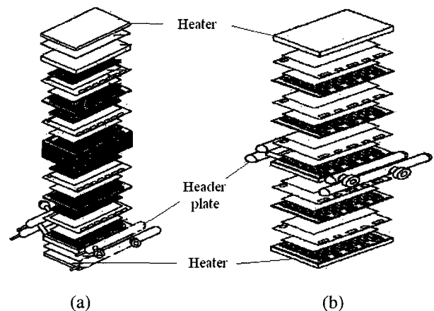
Fig. 1. Schematics of MCFC stack configuration. (a) 6 kW stack, (b) 25 kW stack.
