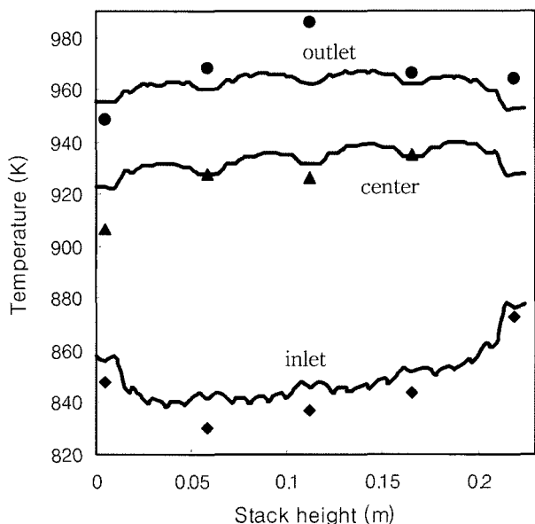
Fig. 6. Temperature distributions compared with experimental data (6 kW, U_F=U_o=0.4 , i=100 mA/cm 2 ).
