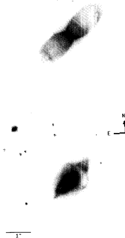
Fig. 4.— Top: He2-320 is an example of PNe with highly collimated lobes. Bottom: A disk can clearly be seen in scattered light in the PPN IRAS 17106–3046.
