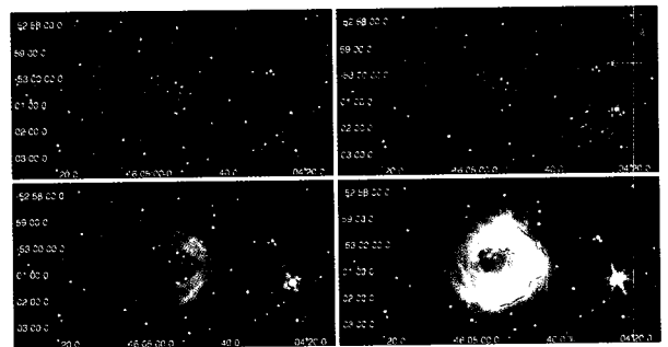
Fig. 2. — A possible PN 329.6-00.4 observed by the GLIMPSE survey of the SST . The four images are 3.6 \mu\text{m} (top left), 4.5 \mu\text{m} (top right), 5.8 \mu\text{m} (bottom left), and 8 \mu\text{m} (bottom right).
