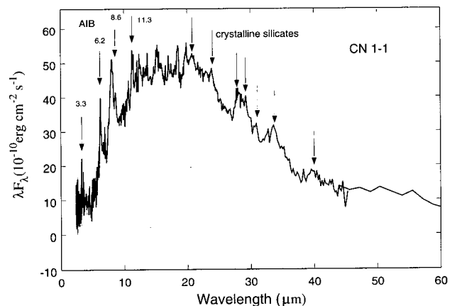
Fig. 7.— ISO SWS01 spectrum of the PN CN1-1 showing the presence of crystalline silicate features as well as aromatic infrared bands at 3.3, 6.2, 7.7, 8.6 and 11.3 \mu\text{m} .
