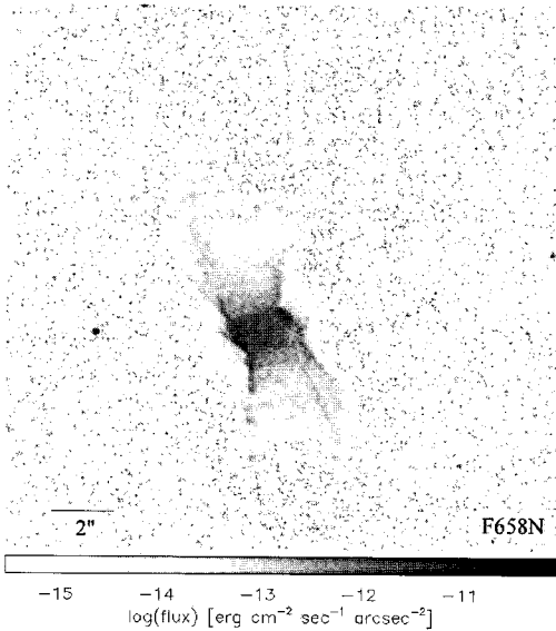
Fig. 6.— A number of 2-D rings can be seen in the lobes of the quadrupolar PN NGC 6881.
