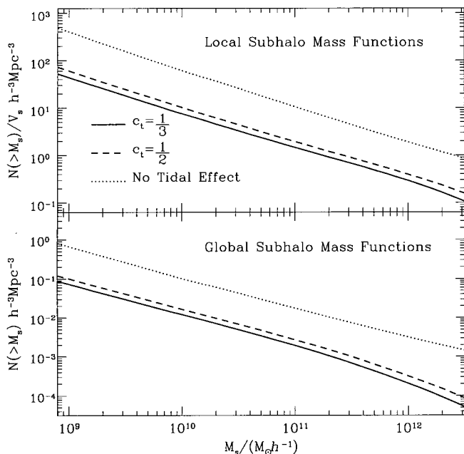
Fig. 1. — The mass functions of the dark halo substructures at redshift z=0 : Upper Panel : the local distribution and Lower Panel : the global distribution. The solid and dashed lines correspond to the two different values of the free parameter c_t in the tidal survival condition (see, eq. [2]). The dotted lines correspond to the case of no tidal stripping effect.
