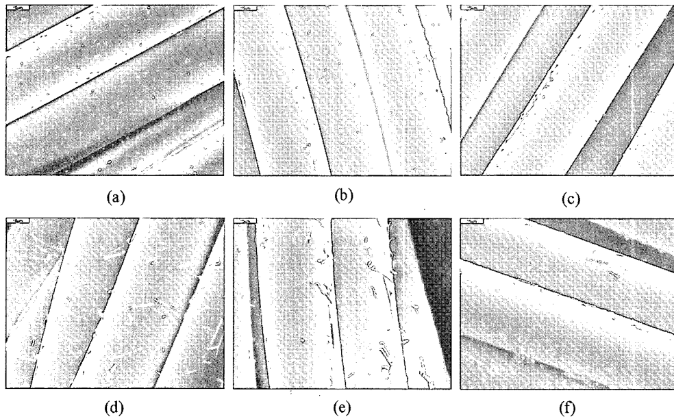
Figure 3. SEM photographs of PTT and PTT fabrics treated by He/O 2 atmospheric pressure plasma: (a) PET control, (b) PET 2 min., (c) PET 4 min., (d) PTT control, (e) PTT 2 min., (f) PTT 4 min.
