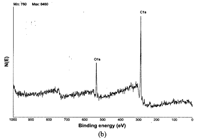
Figure 5. XPS survey scan of PTT warp knitted fabrics treated by He/O 2 atmospheric pressure plasma: (a) control, (b) 2 min.
