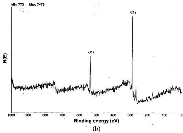
Figure 4. XPS survey scan of PET warp knitted fabrics treated by He/O 2 atmospheric pressure plasma: (a) control, (b) 2 min.
