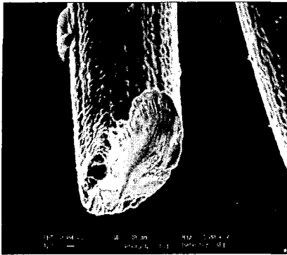
Fig. 5 Fracture by initial defect
