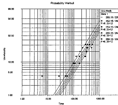
Fig. 11 Weibull probability plot for test data
