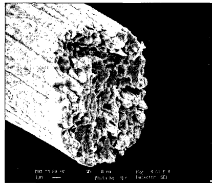
Fig. 4 Brittle fracture due to inhomogeneous distribution of potassium dopant
