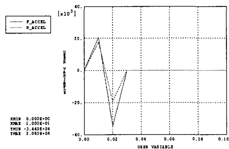
Fig. 7 Impact data measured when closing the door
