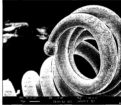
Fig. 2 Hot spot burnout of tungsten filament
