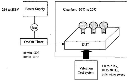
Fig. 10 Schematic diagram for test system
