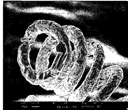
Fig. 3 Sag due to recrystallization and growth
