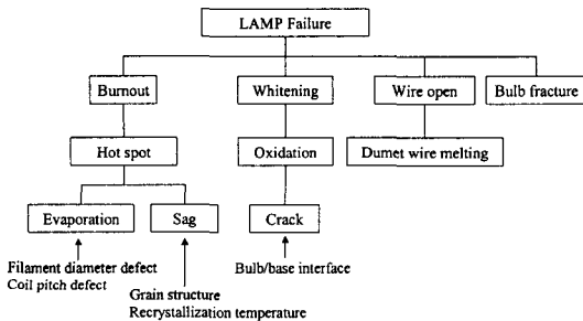
Fig. 1 Failure modes and mechanisms of lamp
