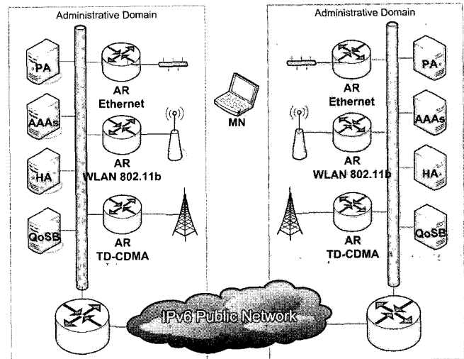
Fig. 2. The Moby Dick "True-IP" architecture.
